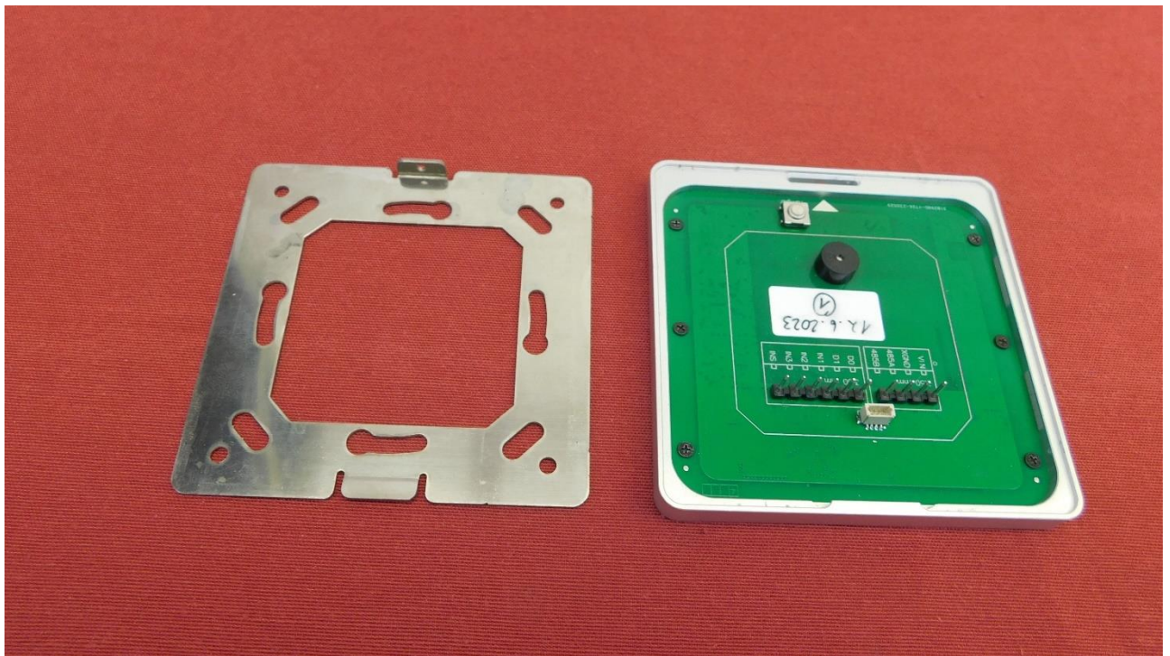
Picture 3: EUT – rear view with unmounted support
