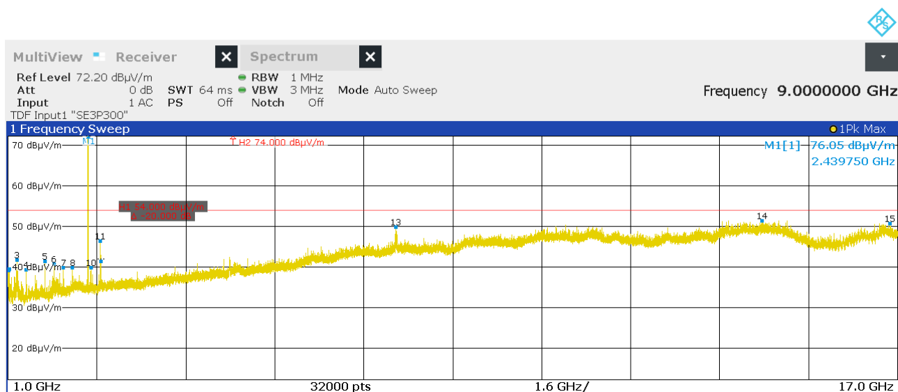
Figure 37: Chart of radiated emissions pre-measurement from 1 GHz to 17 GHz on middle channel, EUT position Y, antenna polarization vertical
