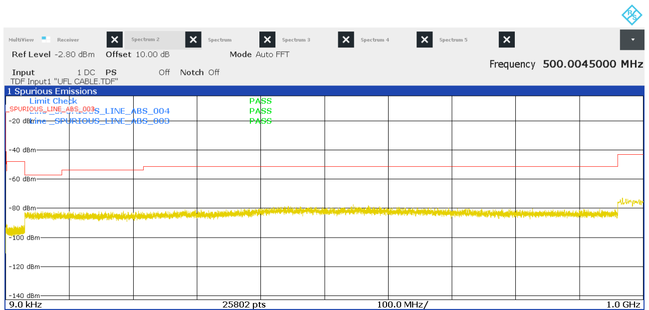
Figure 30: Chart of emissions test from 9 kHz to 1 GHz on highest channel, PK
