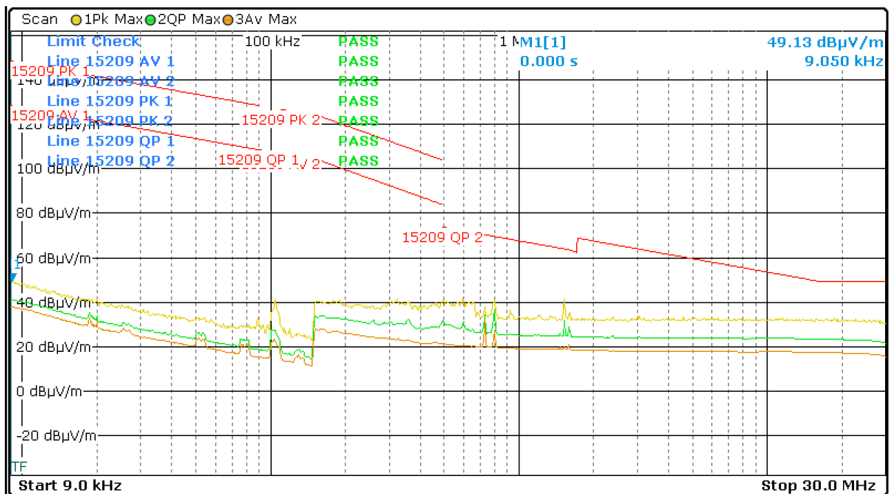
Figure 33: Chart of emissions test below 30 MHz on lowest channel, EUT position Y, antenna parallel
