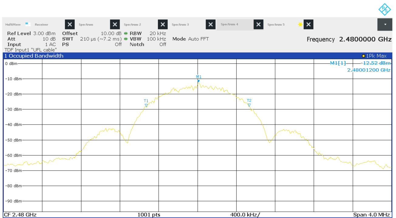
Figure 14: Chart of occupied bandwidth test on highest channel
