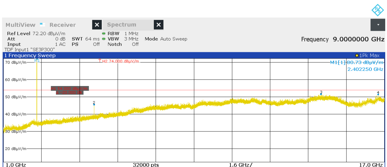
Figure 35: Chart of radiated emissions pre-measurement from 1 GHz to 17 GHz on lowest channel, EUT position Y, antenna polarization horizontal
