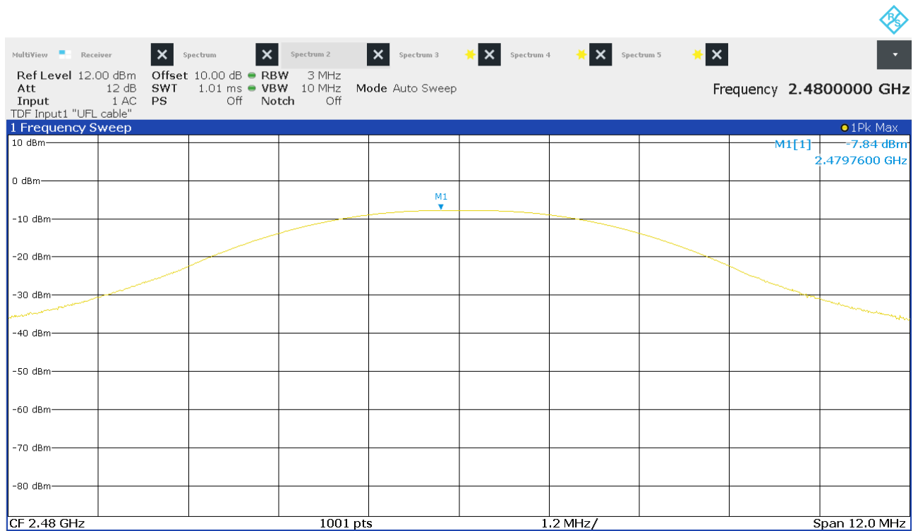
Figure 17: Chart of conducted output power on highest channel
