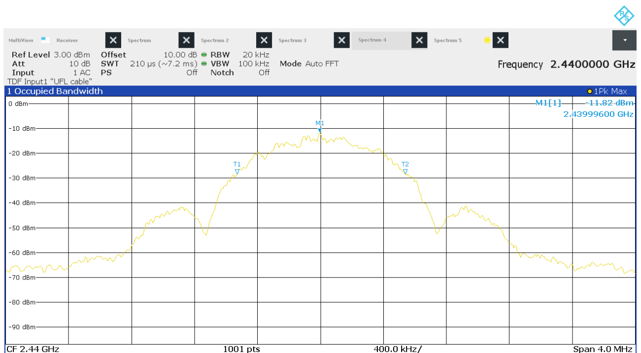
Figure 13: Chart of occupied bandwidth test on middle channel
