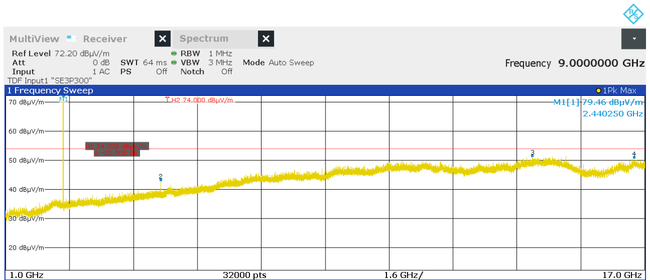
Figure 37: Chart of radiated emissions pre-measurement from 1 GHz to 17 GHz on middle channel, EUT position Y, antenna polarization horizontal
