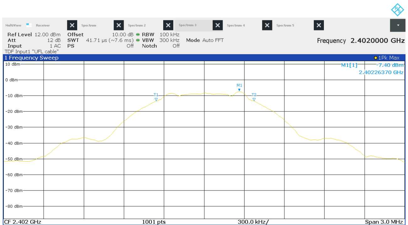
Figure 9: Chart of 6 dB bandwidth test on lowest channel
