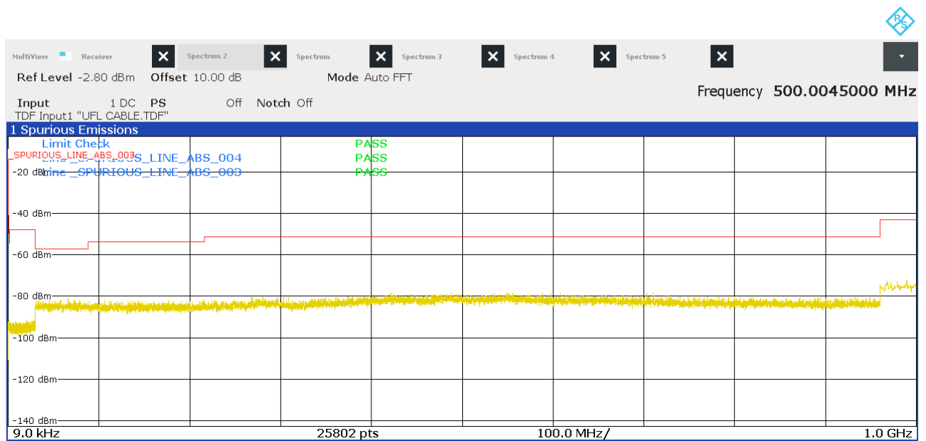
Figure 27: Chart of emissions test from 9 kHz to 1 GHz on middle channel, PK
