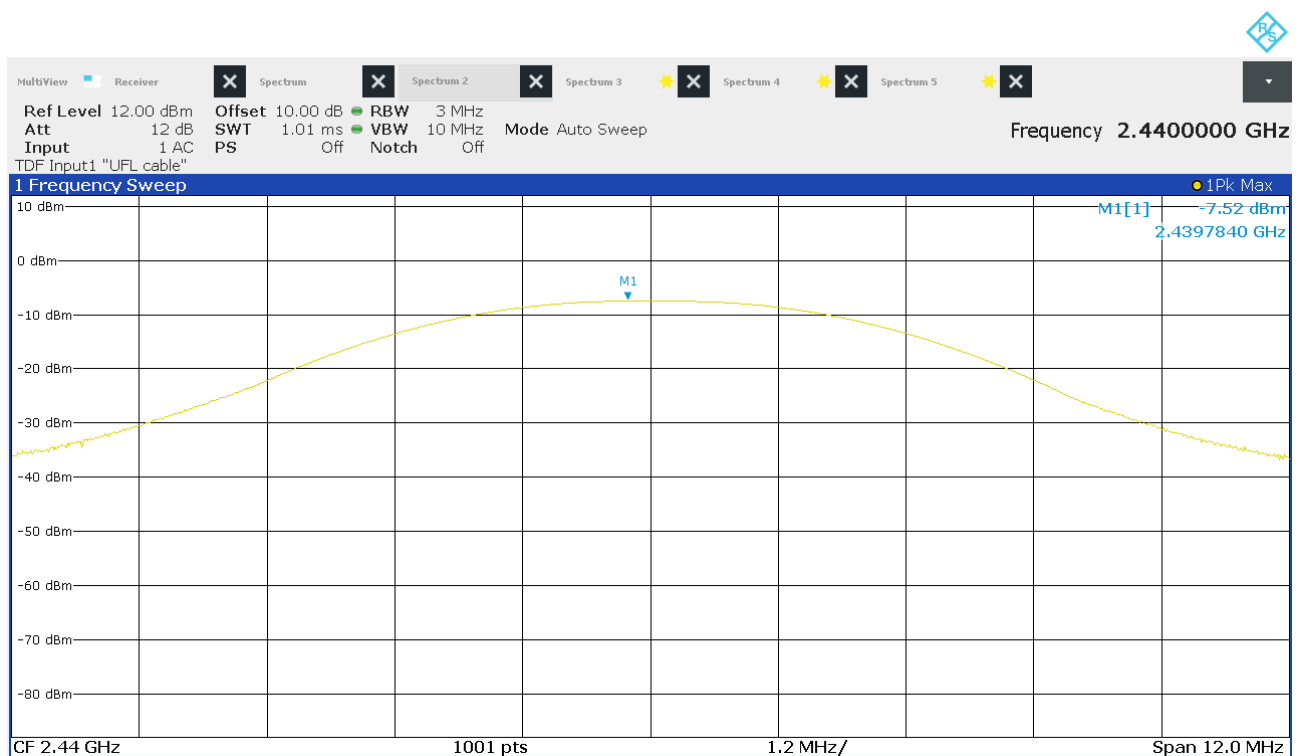
Figure 16: Chart of conducted output power on middle channel
