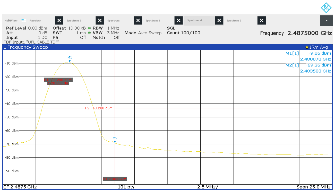
Figure 23: Chart of upper band-edge measurement on highest channel (RMS)
