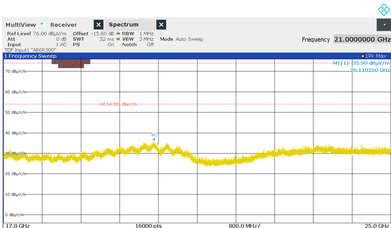
Figure 40: Chart of exploratory emission test from 17 GHz to 25 GHz on highest channel, EUT position Y, antenna polarization vertical
