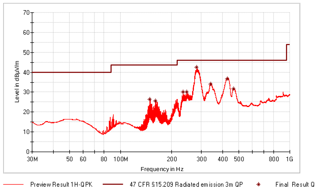
Figure 34: Chart of radiated emissions test from 30 MHz to 1 GHz on middle channel, EUT position Y, antenna polarization horizontal
