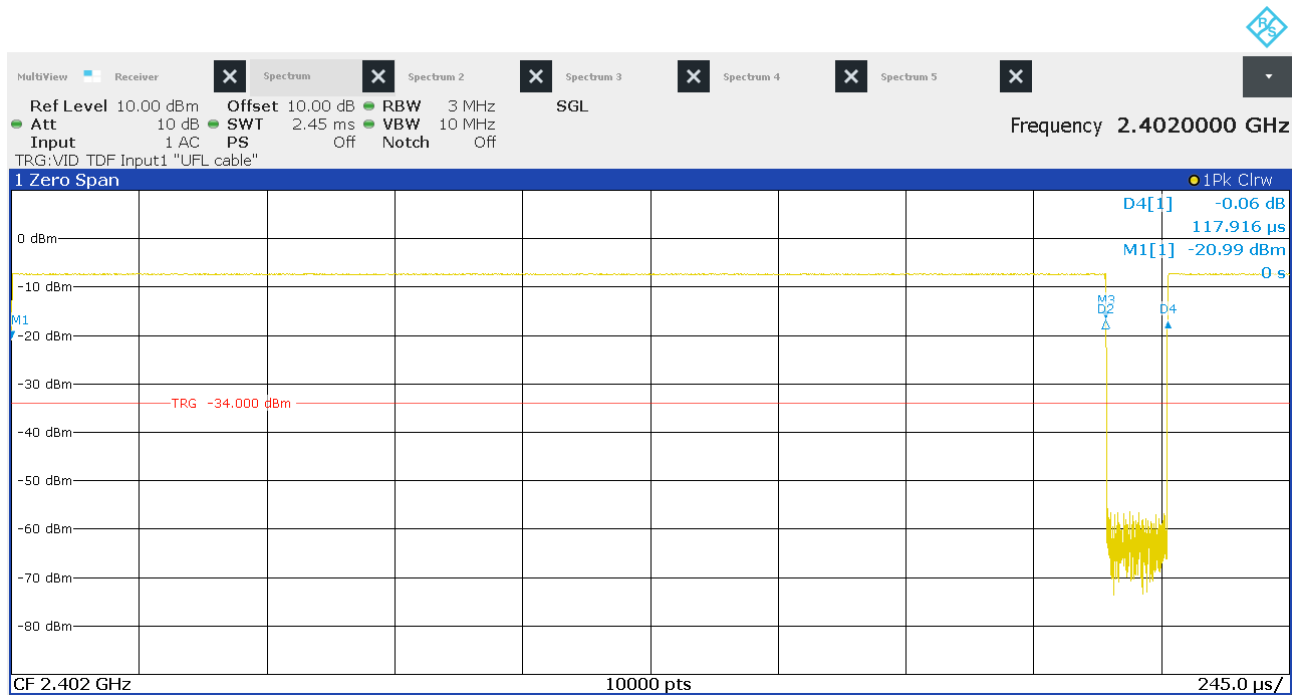
Figure 8: Chart of duty cycle test on lowest channel
