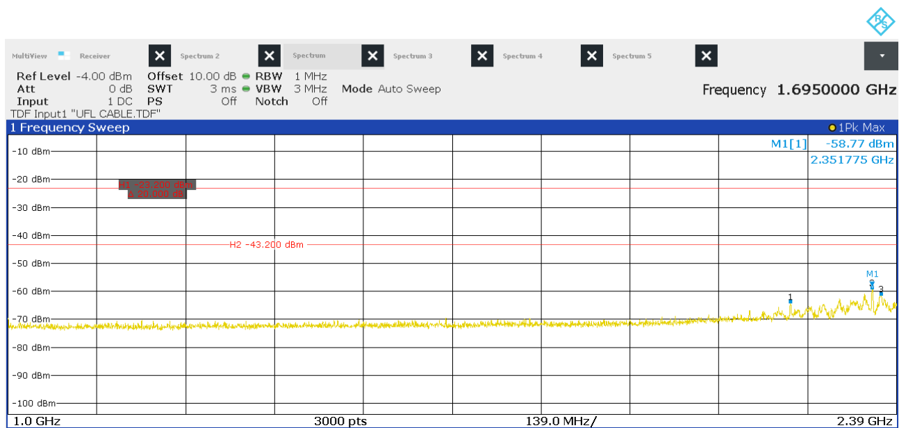
Figure 31: Chart of emissions test from 1 GHz to 2.39 GHz on highest channel, Pk
