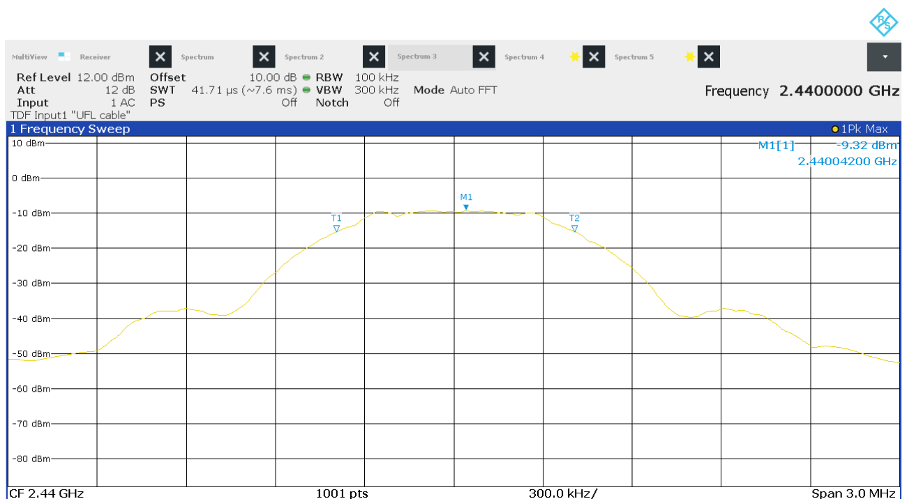
Figure 10: Chart of 6 dB bandwidth test on middle channel
