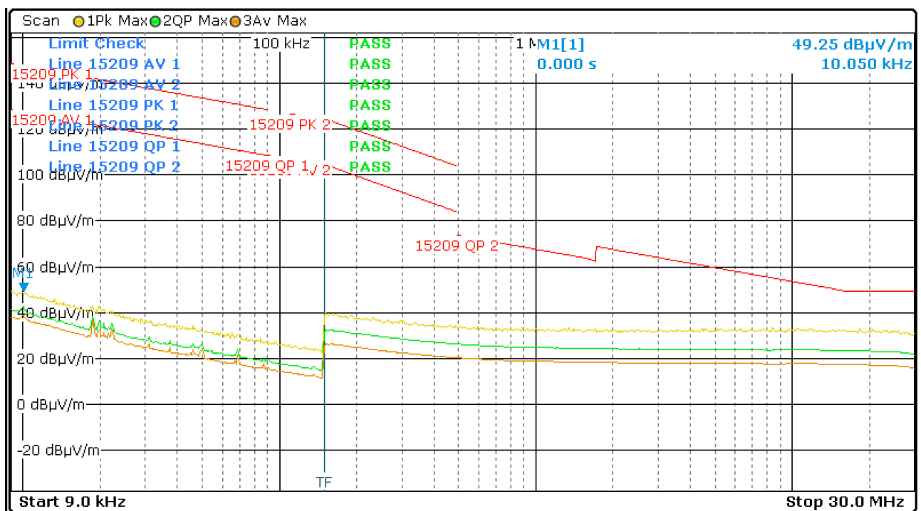
Figure 33: Chart of emissions test below 30 MHz on lowest channel, EUT position Y, antenna in line
