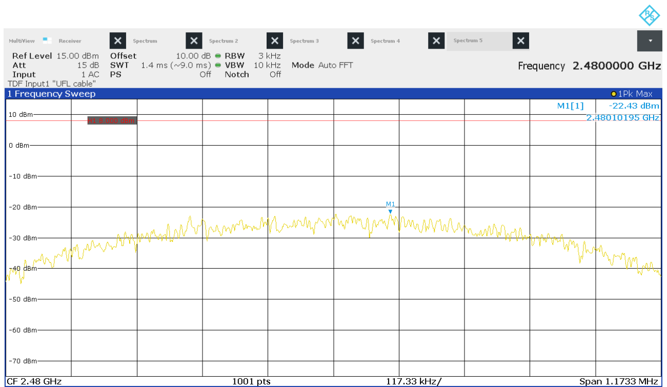
Figure 20: Chart of power spectral density on highest channel
