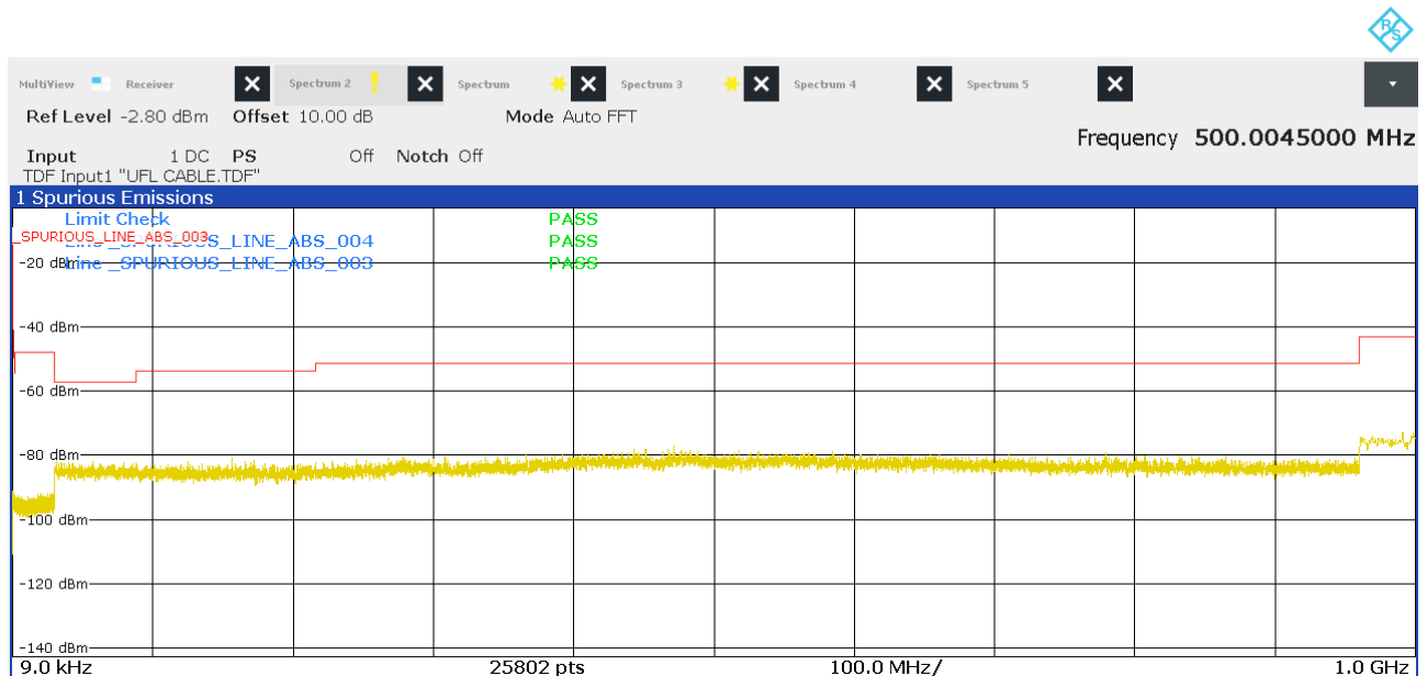
Figure 24: Chart of emissions test from 9 kHz to 1 GHz on lowest channel, PK
