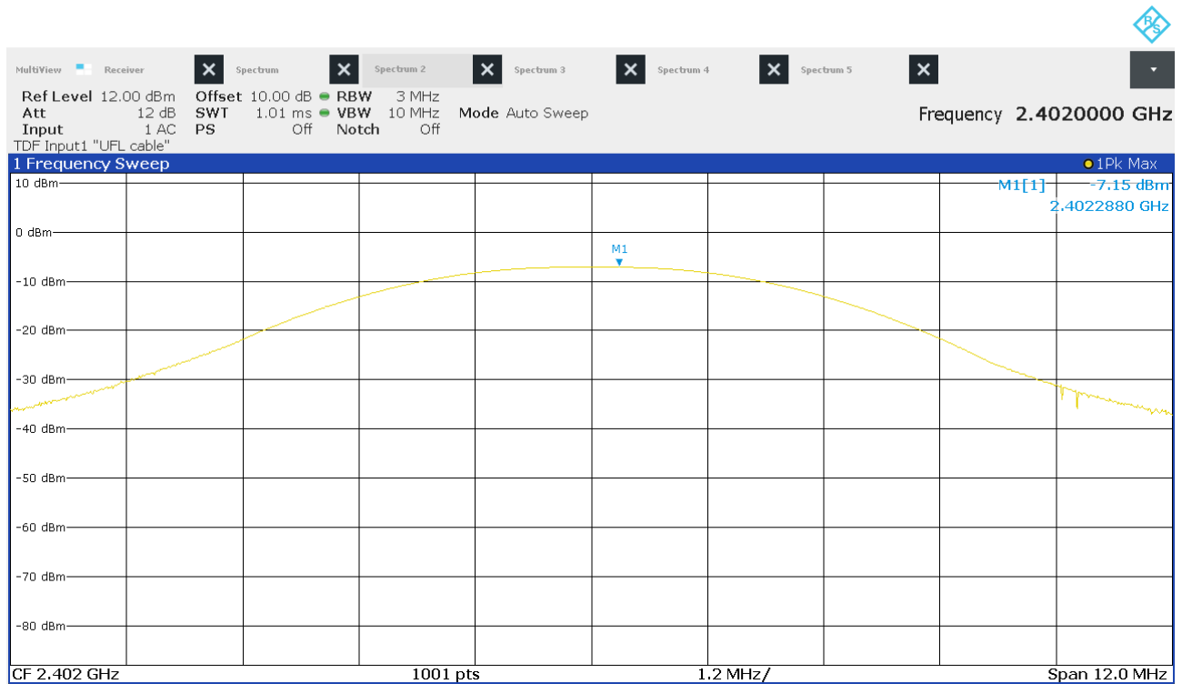
Figure 15: Chart of conducted output power on lowest channel
