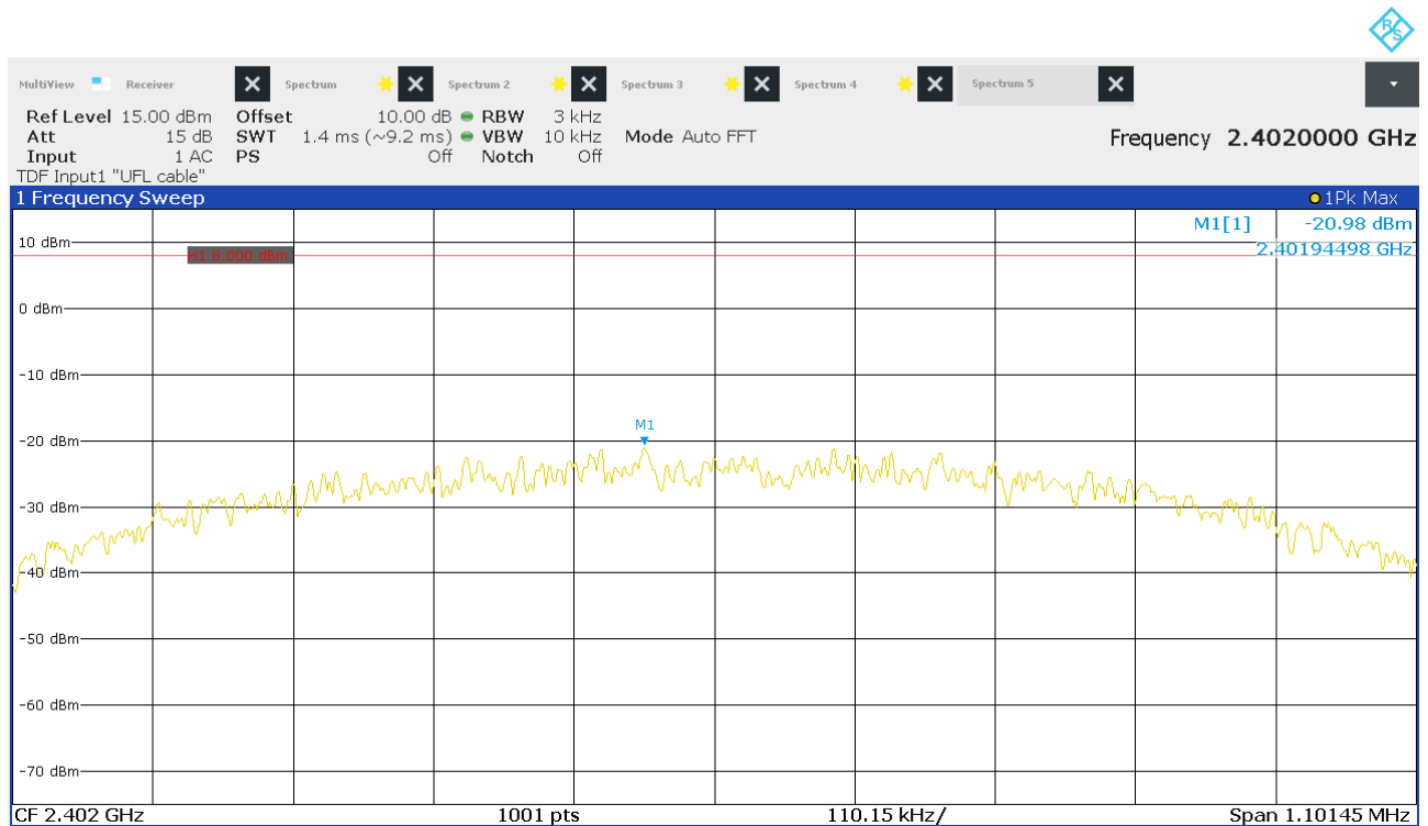
Figure 18: Chart of power spectral density on lowest channel
