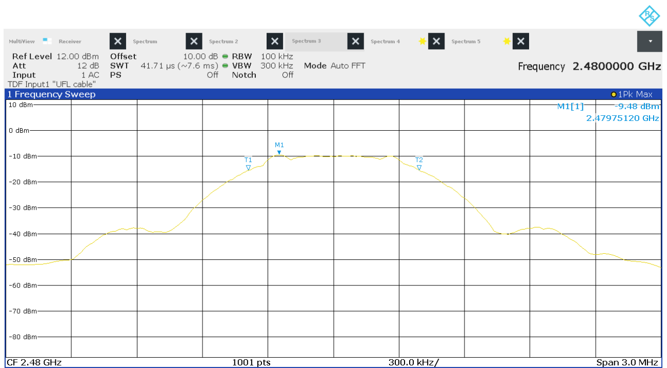
Figure 11: Chart of 6 dB bandwidth test on highest channel
