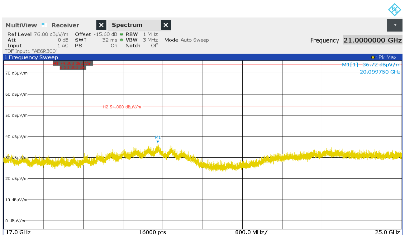
Figure 38: Chart of exploratory emissions measurement from 17 GHz to 25 GHz on middle channel, EUT position Y, antenna polarization vertical
