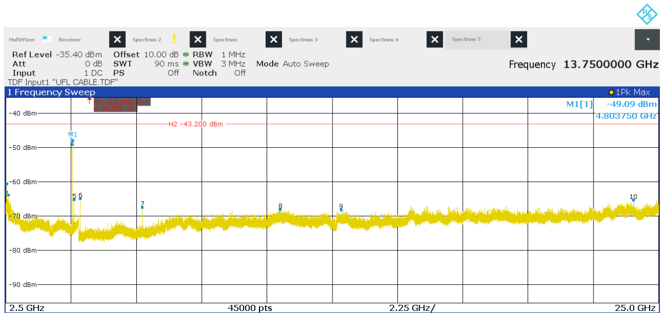
Figure 26: Chart of emissions test from 2.5 GHz to 25 GHz on lowest channel, Pk
