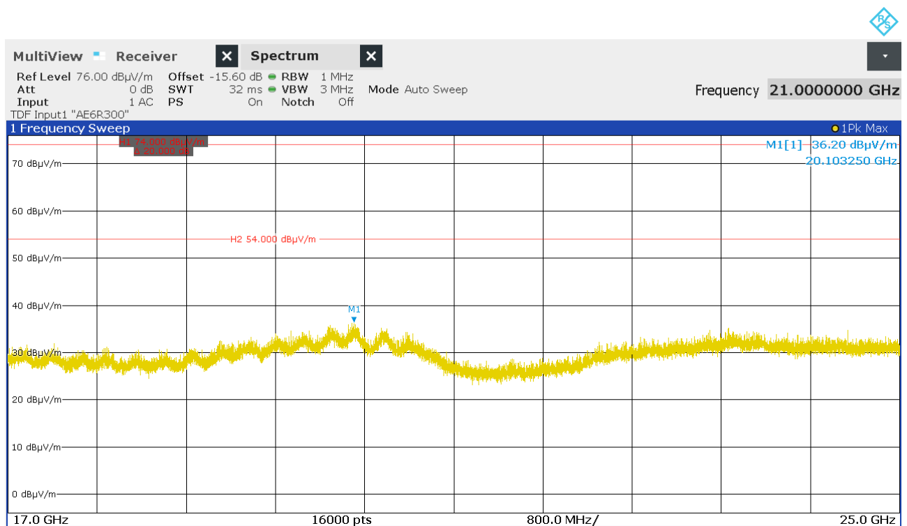
Figure 36: Chart of exploratory radiated emissions measurement from 17 GHz to 25 GHz on lowest channel, EUT position Y, antenna polarization vertical
