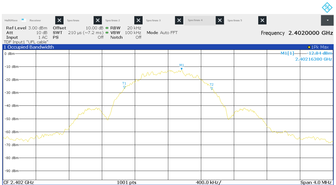
Figure 12: Chart of occupied bandwidth test on lowest channel
