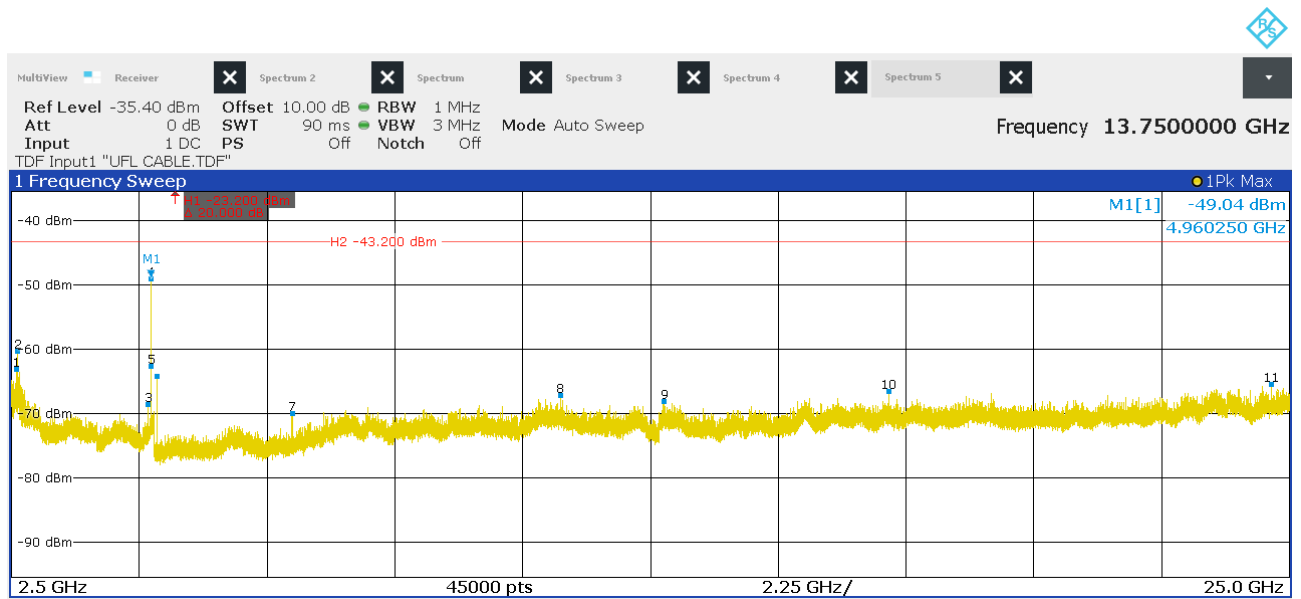
Figure 32: Chart of emissions test from 2.5 GHz to 25 GHz on highest channel, Pk
