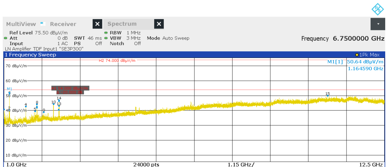
Figure 10: Chart of radiated emissions pre-measurement from 1 GHz to 12.5 GHz, EUT position Y, with tag, antenna polarization vertical
