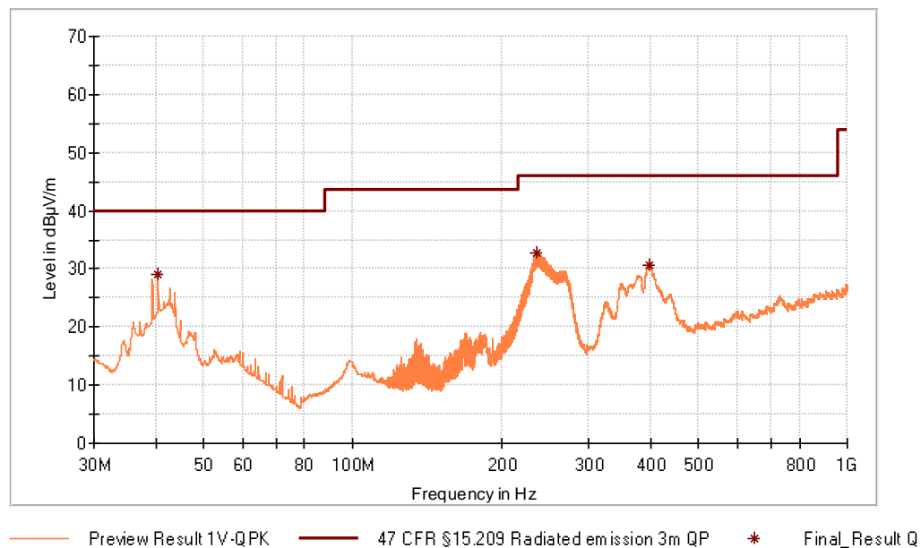
Figure 9: Chart of radiated emissions test from 30 MHz to 1 GHz, EUT position Y, with tag, antenna vertical
