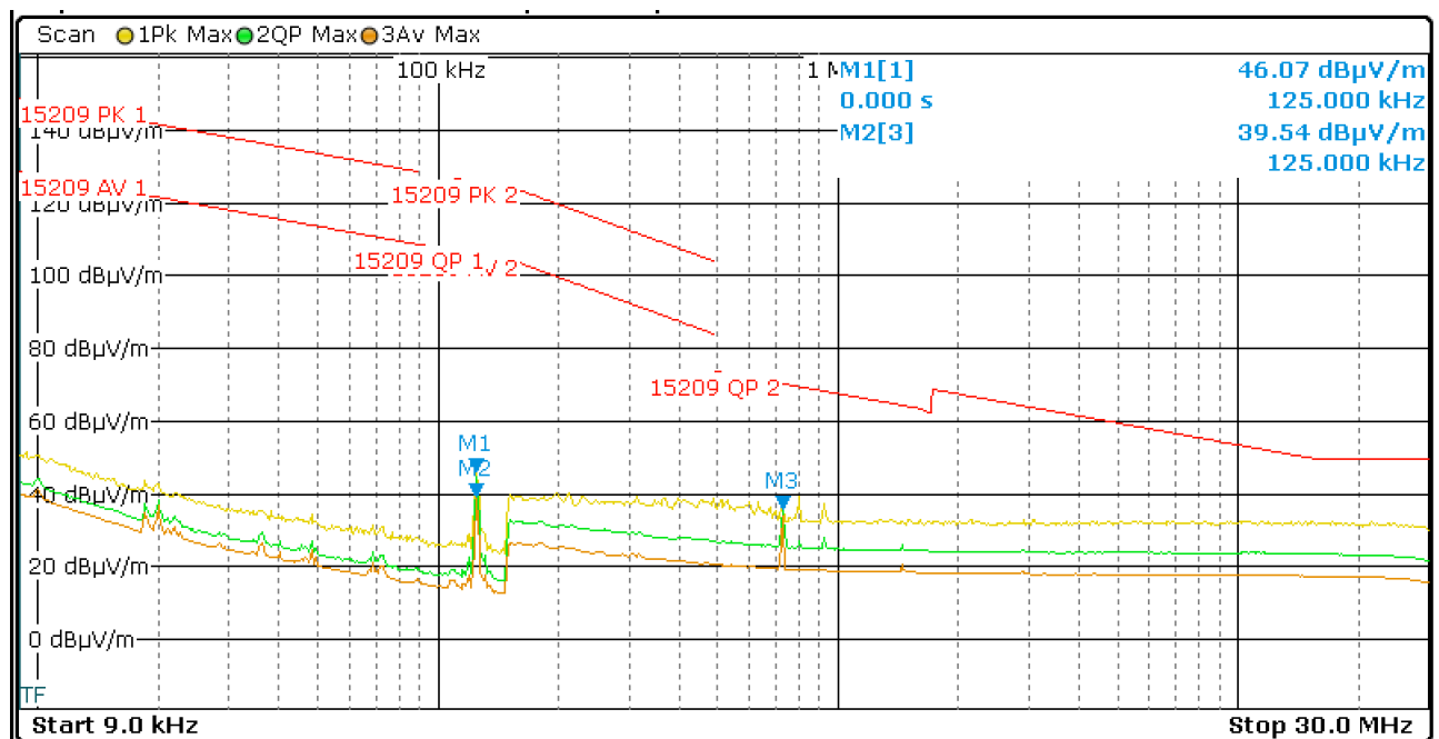
Figure 8: Chart of radiated emissions test below 30 MHz, EUT position Y, antenna polarization in line, with tag
