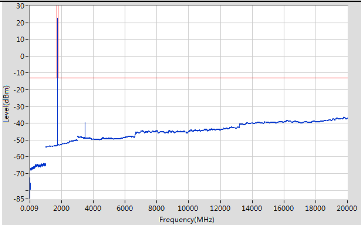
Band66_3MHz_16QAM_132322_1RB#0
