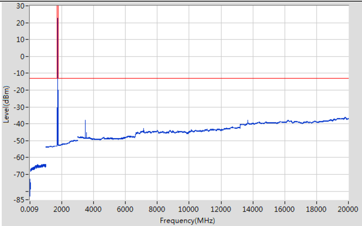
Band66_15MHz_16QAM_132322_1RB#38
