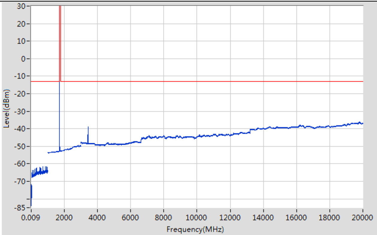
Band66_3MHz_16QAM_131987_1RB#0
