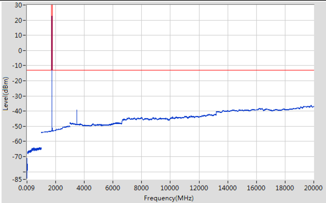
Band66_5MHz_16QAM_132322_1RB#13
