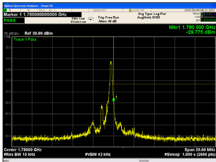
Band66-1.4MHz-QPSK-132665-1RB#5
