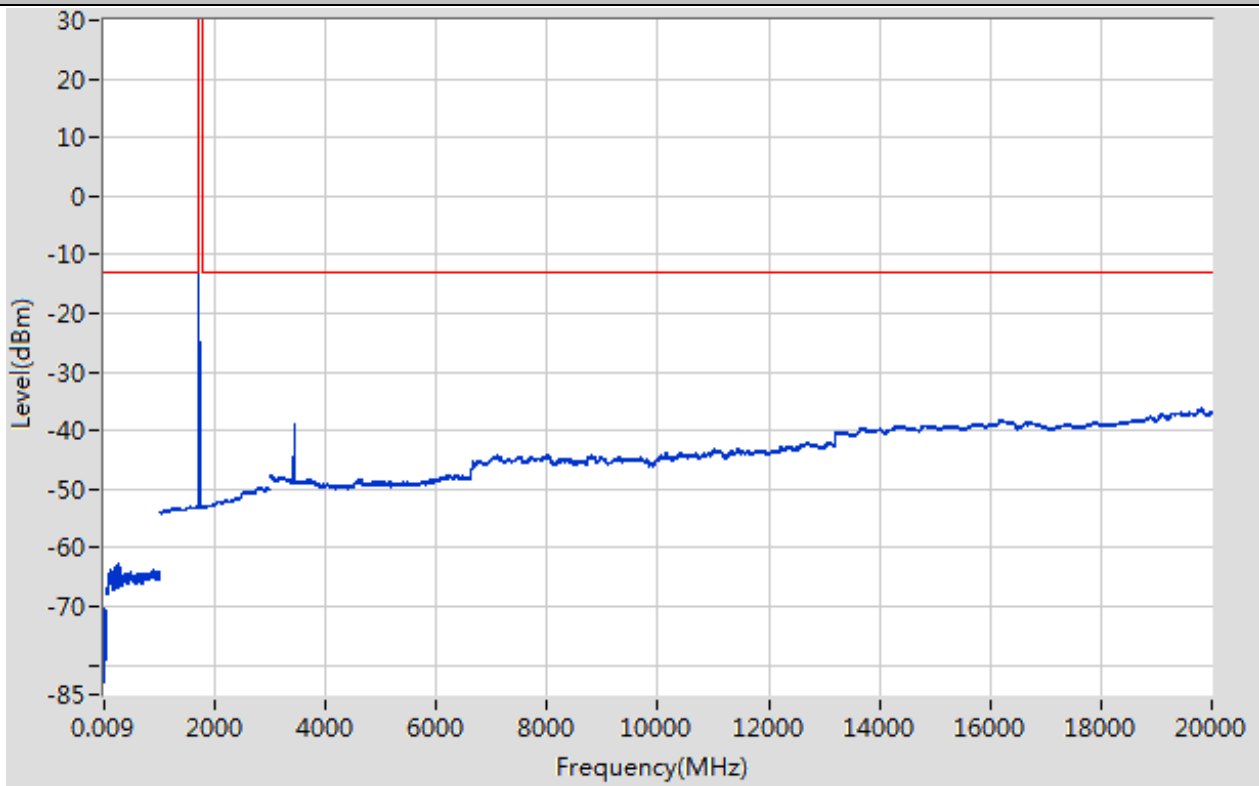
Band66_5MHz_16QAM_131997_1RB#13
