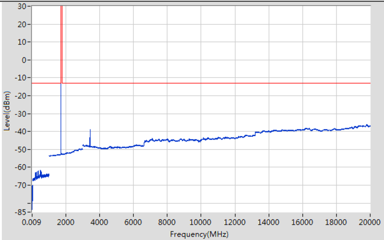
Band66_1.4MHz_16QAM_131979_3RB#2
