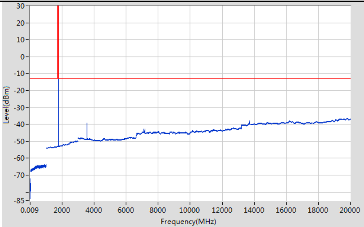
Band66_1.4MHz_16QAM_132665_3RB#2
