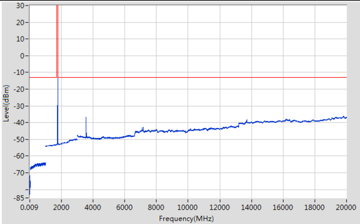
Band66_10MHz_16QAM_132622_1RB#49
