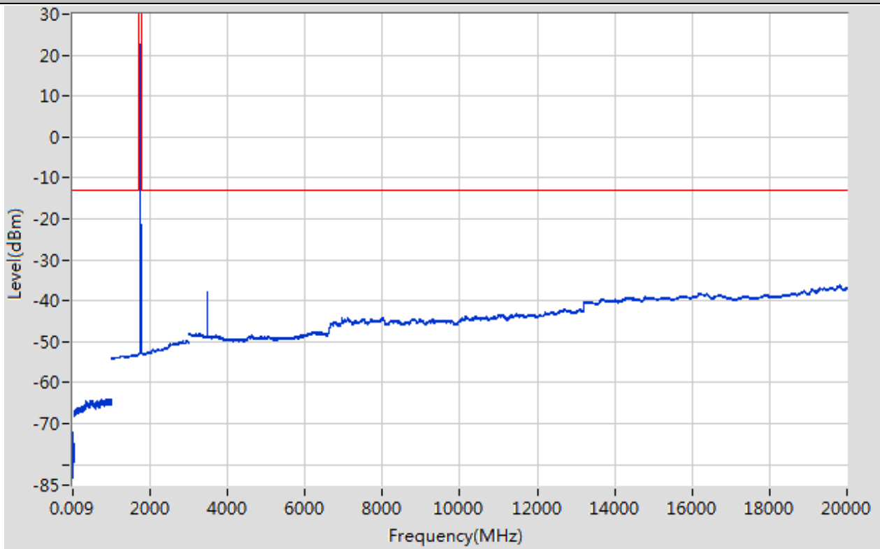
Band66_10MHz_16QAM_132322_1RB#49
