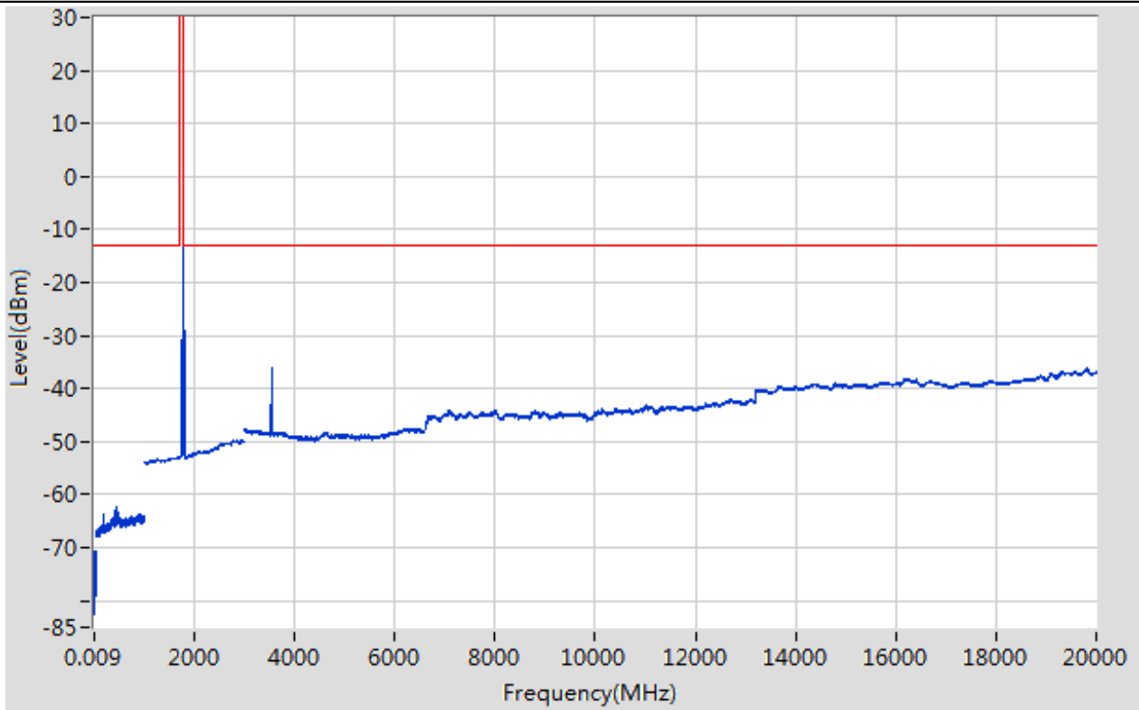
Band66_15MHz_16QAM_132597_1RB#38
