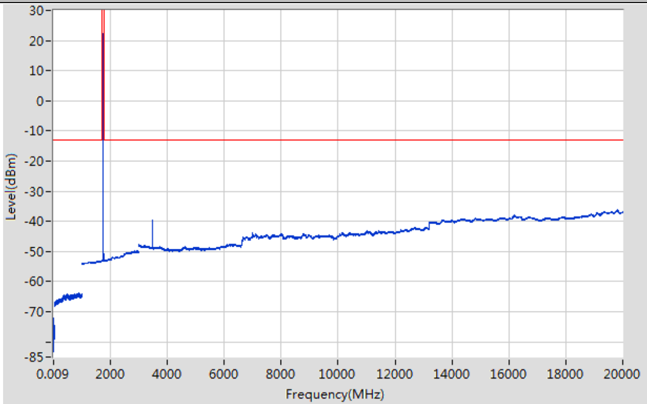
Band66_5MHz_16QAM_132322_1RB#13
