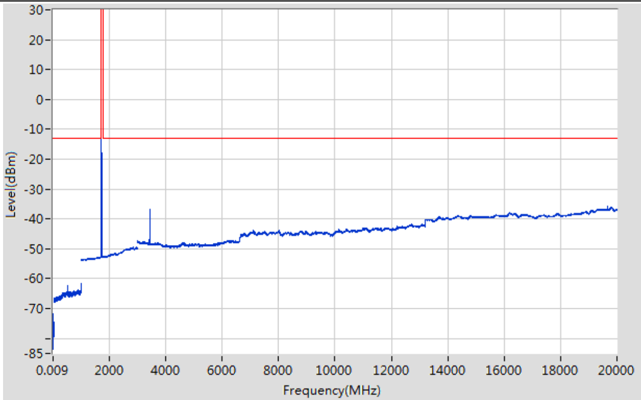
Band66_10MHz_16QAM_132022_1RB#49
