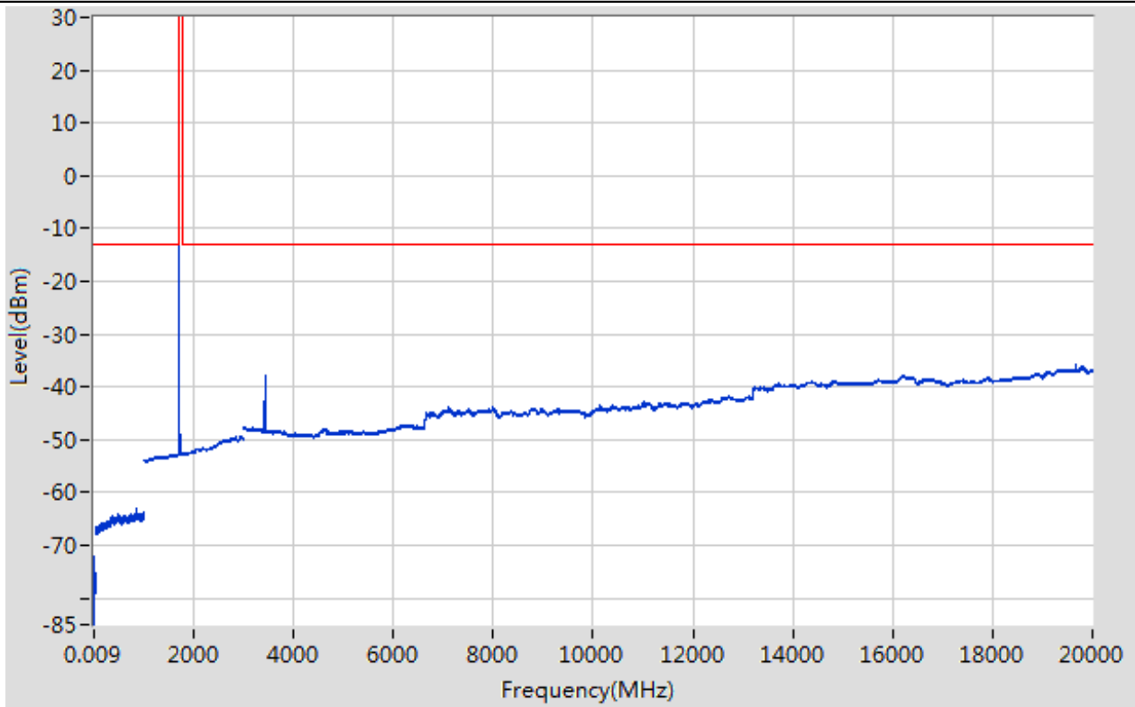
Band66_3MHz_16QAM_131987_1RB#0
