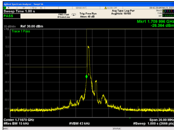
Band66-1.4MHz-QPSK-131979-6RB#0
