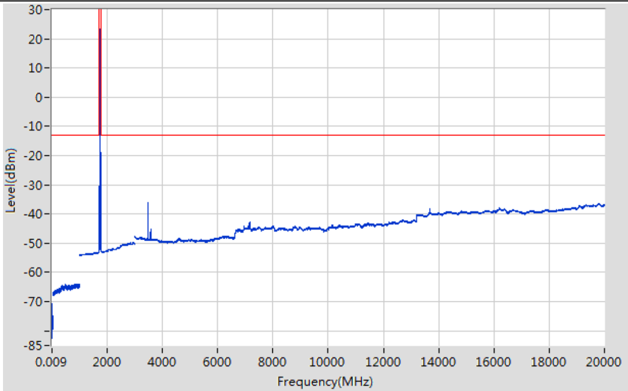
Band66_20MHz_16QAM_132322_1RB#50
