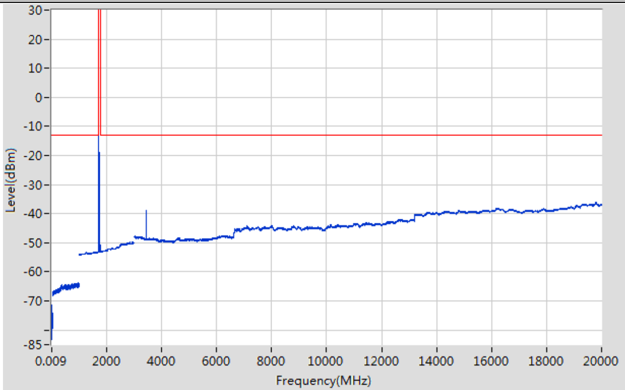
Band66_15MHz_16QAM_132047_1RB#38
