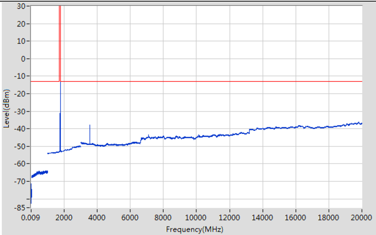
Band66_10MHz_16QAM_132622_1RB#49
