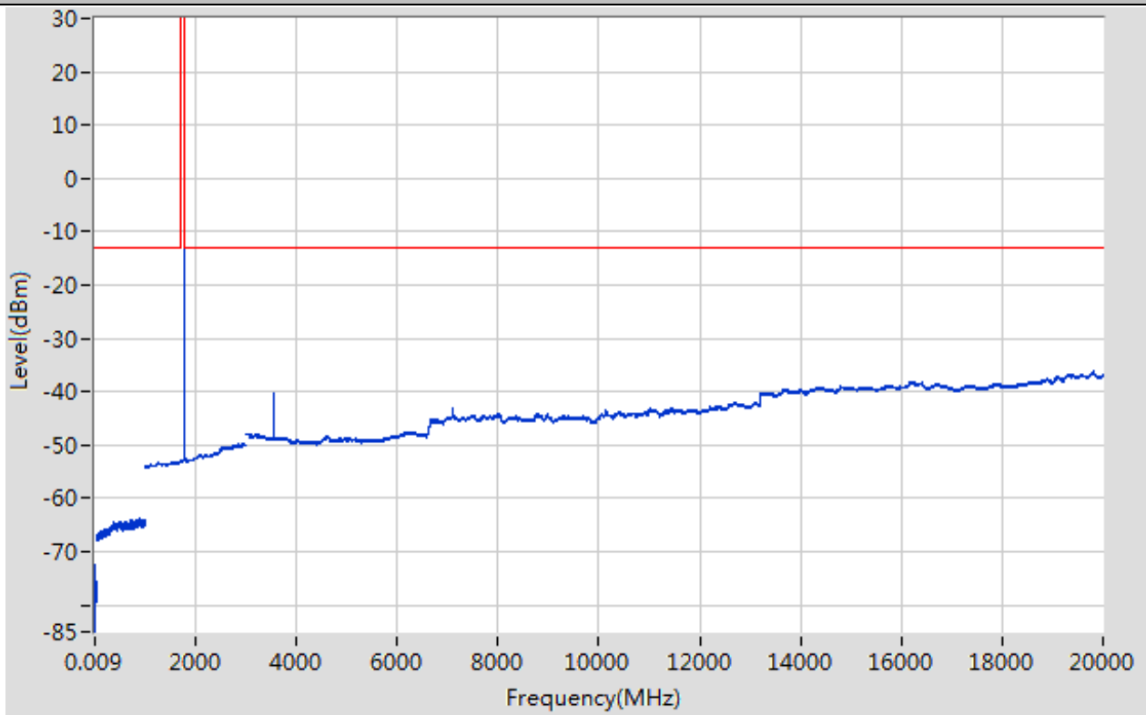
Band66_3MHz_16QAM_132657_1RB#0
