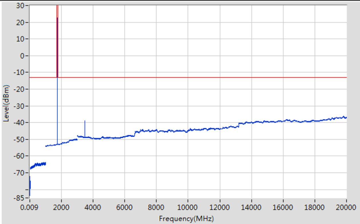
Band66_1.4MHz_16QAM_132322_3RB#2
