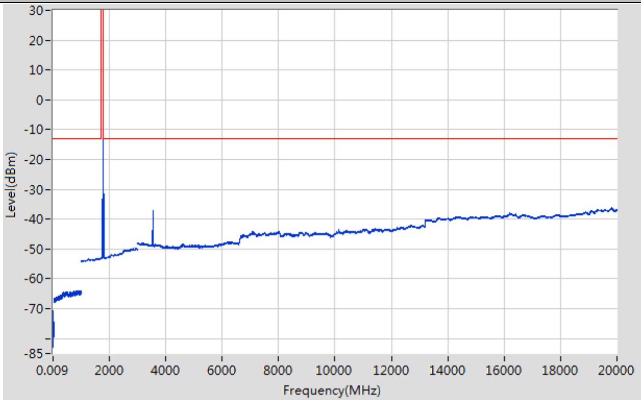
Band66_15MHz_16QAM_132597_1RB#38
