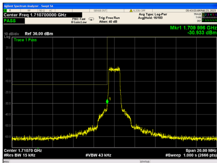
Band66-1.4MHz-QPSK-132665-1RB#5
