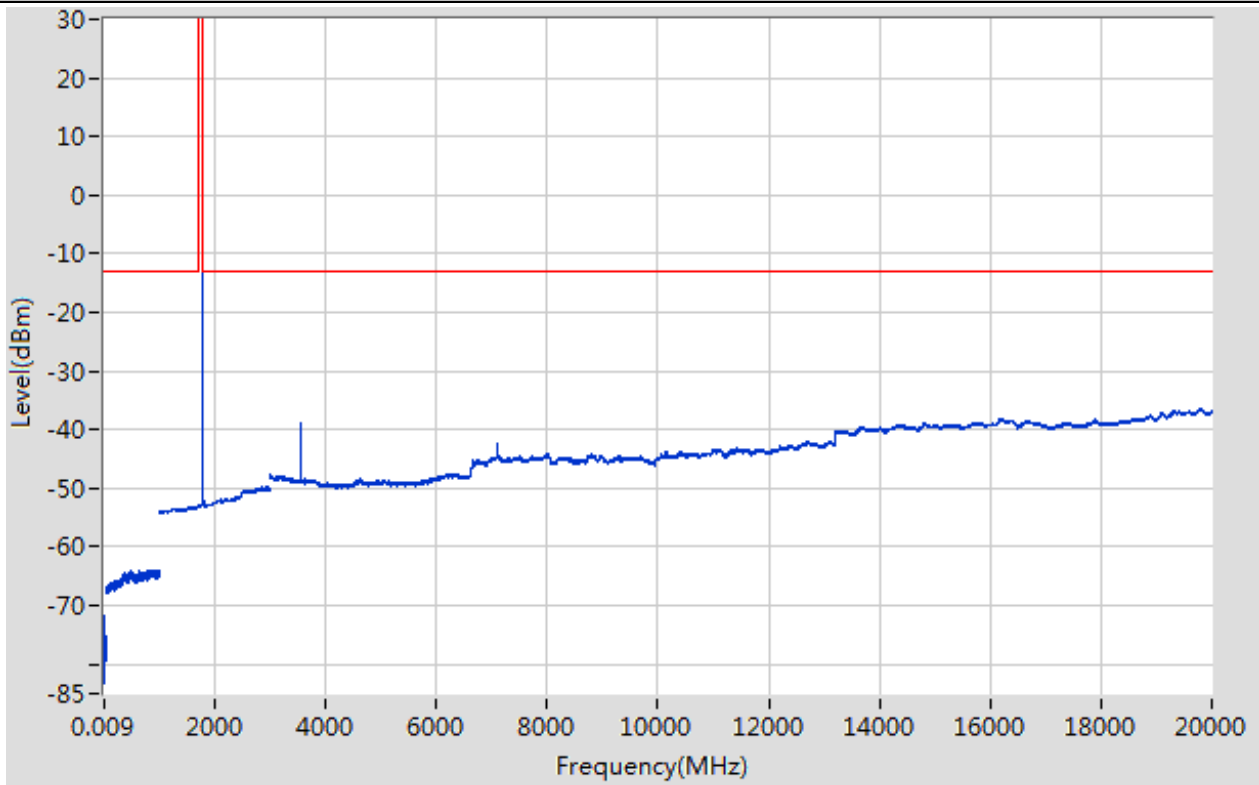
Band66_5MHz_16QAM_132647_1RB#13
