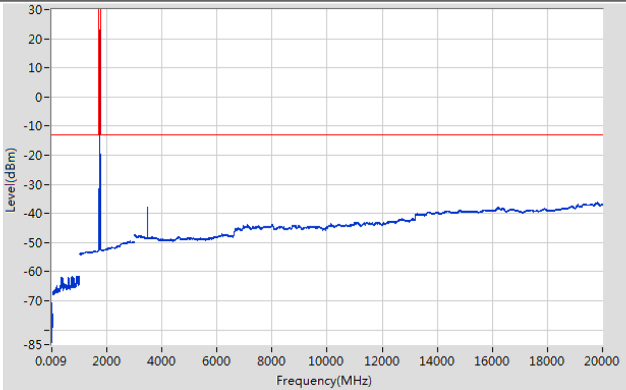
Band66_15MHz_16QAM_132322_1RB#38
