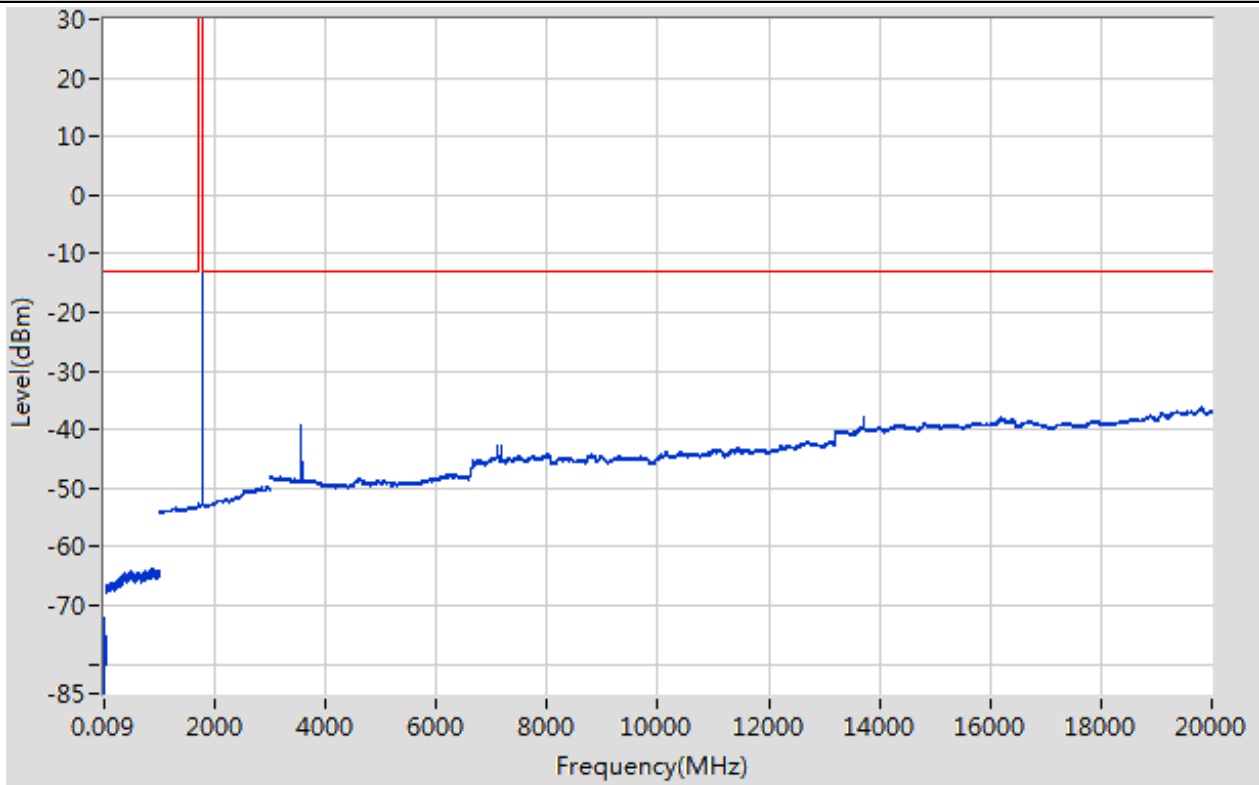
Band66_3MHz_16QAM_132657_1RB#0
