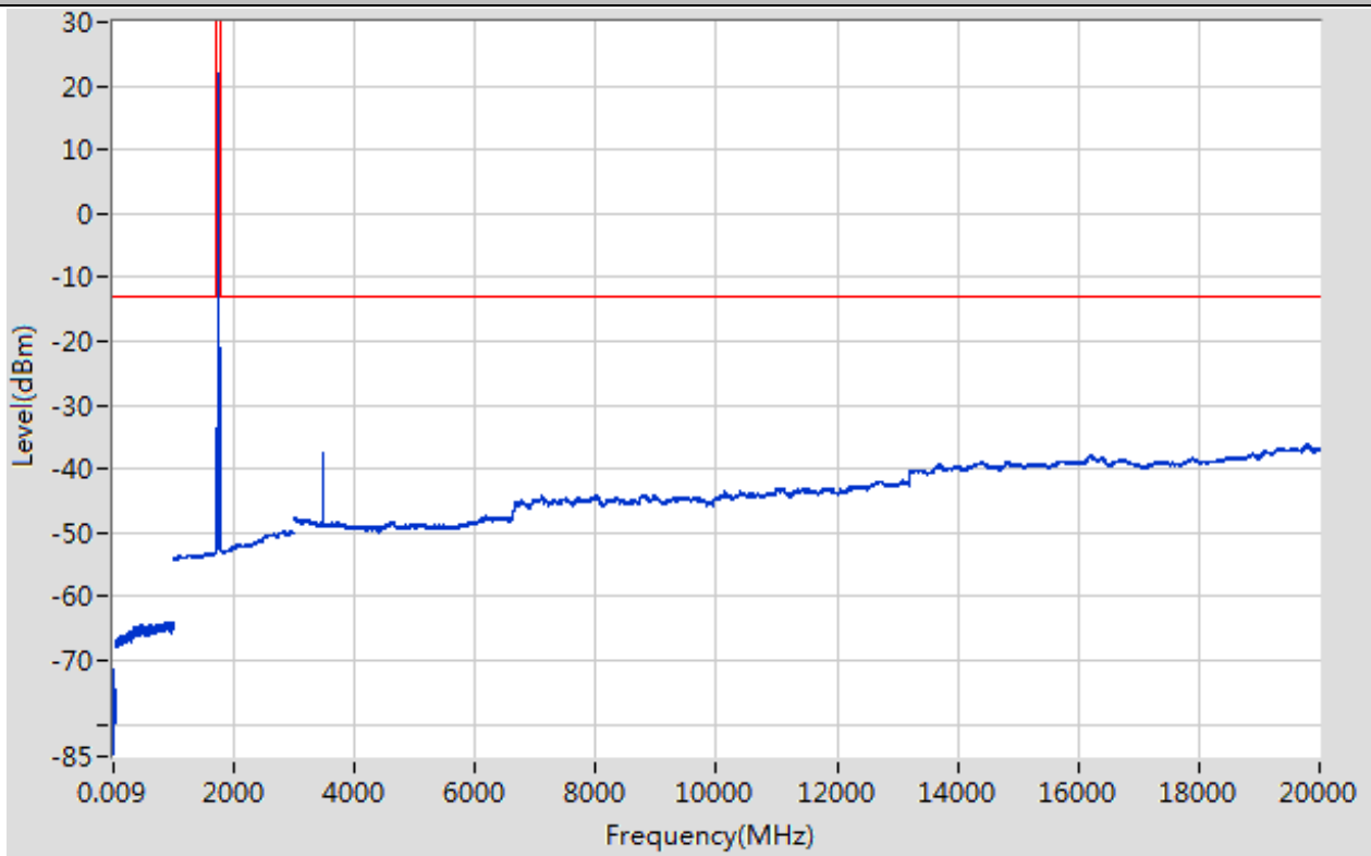
Band66_20MHz_16QAM_132322_1RB#50
