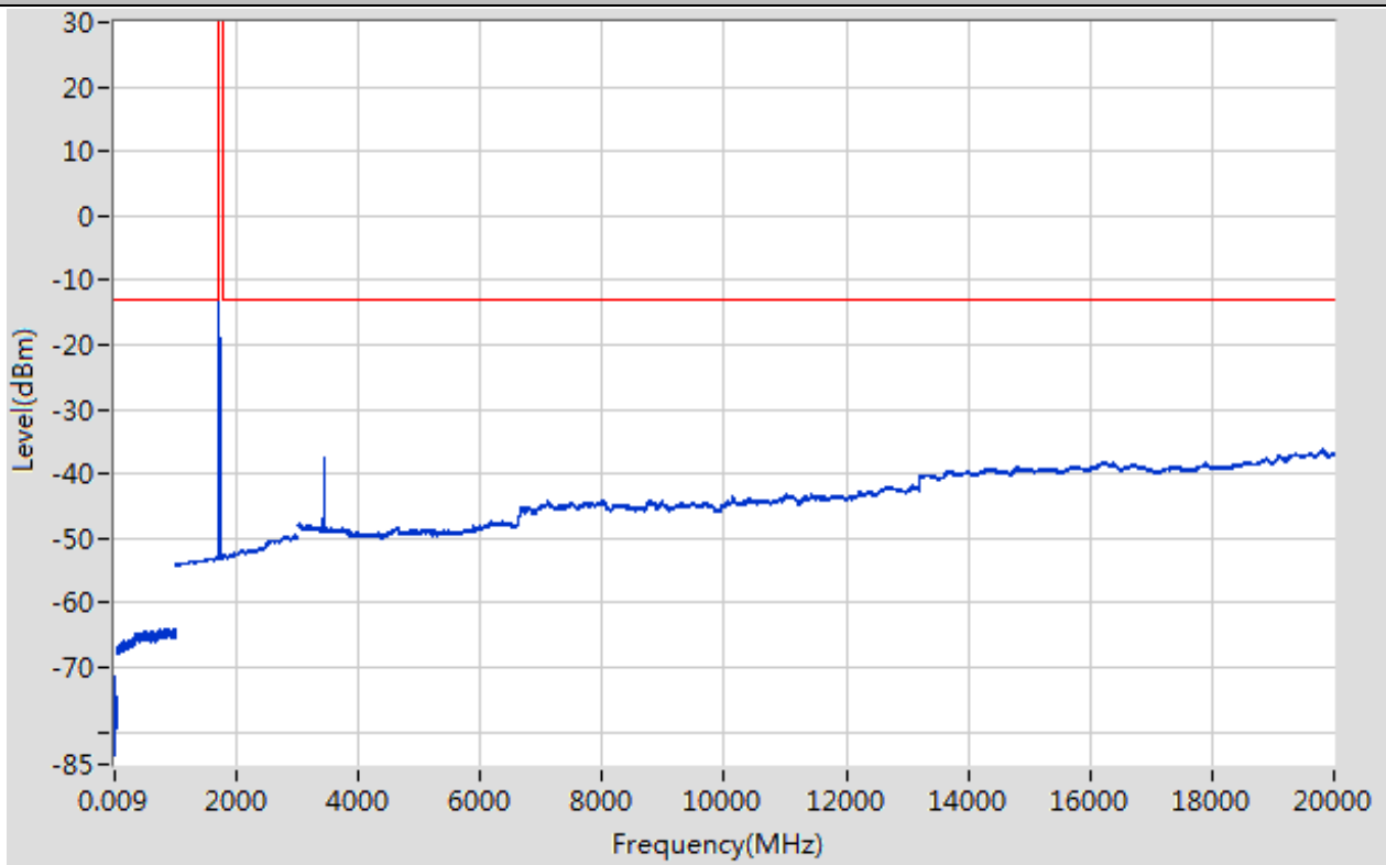
Band66_10MHz_16QAM_132022_1RB#49
