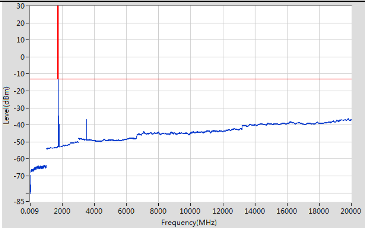
Band66_20MHz_16QAM_132572_1RB#50
