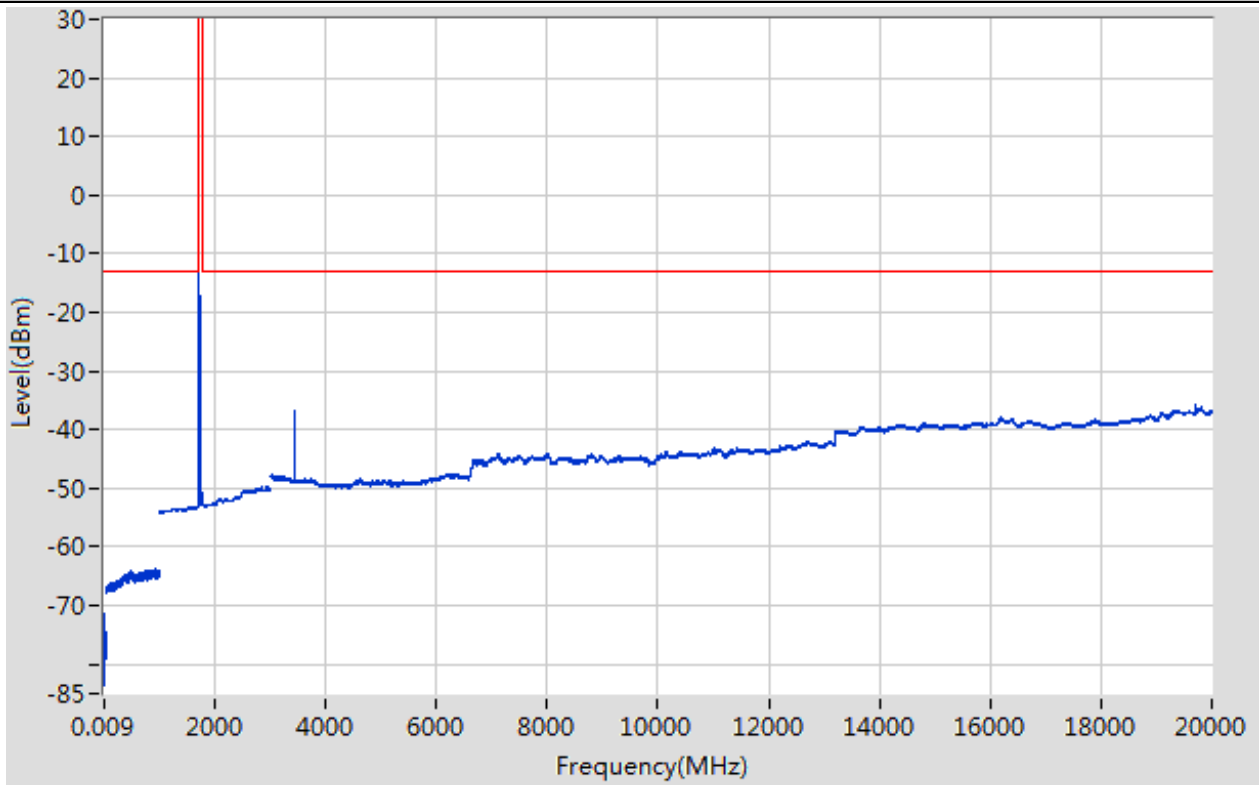
Band66_20MHz_16QAM_132072_1RB#50
