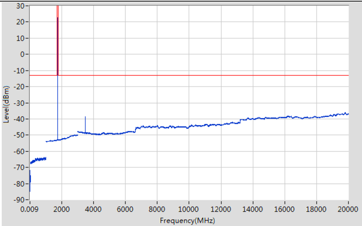
Band66_1.4MHz_16QAM_132322_3RB#2
