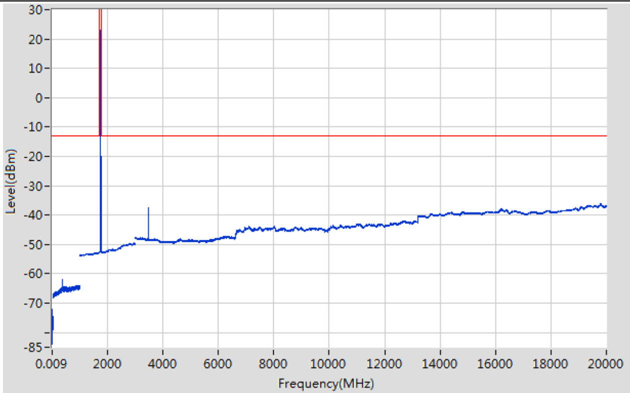
Band66_10MHz_16QAM_132322_1RB#49
