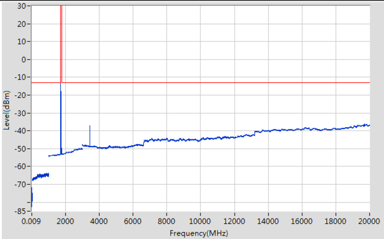
Band66_15MHz_16QAM_132047_1RB#38
