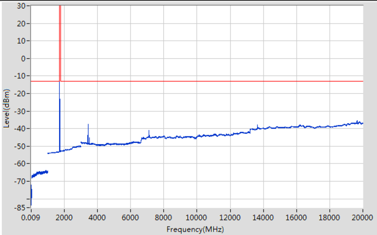
Band66_5MHz_16QAM_131997_1RB#13
