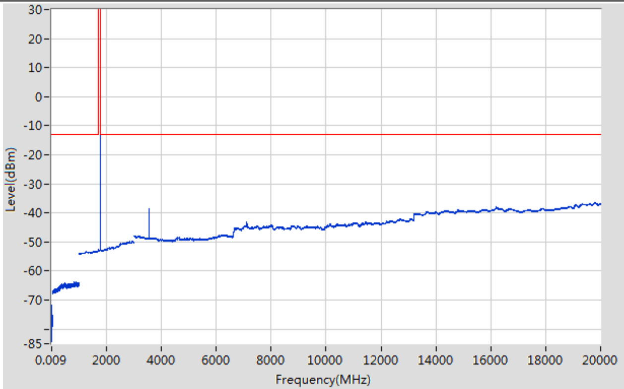
Band66_1.4MHz_16QAM_132665_3RB#2
