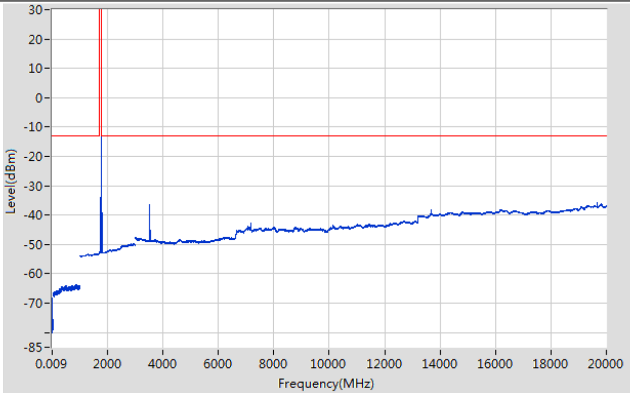
Band66_20MHz_16QAM_132572_1RB#50
