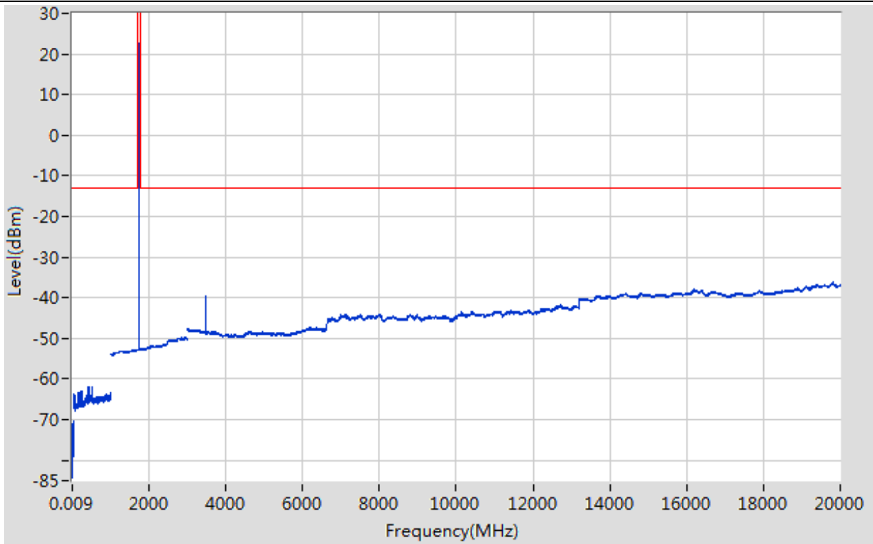
Band66_3MHz_16QAM_132322_1RB#0
