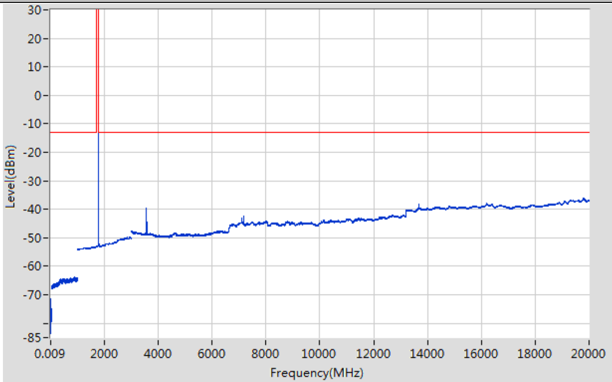
Band66_5MHz_16QAM_132647_1RB#13
