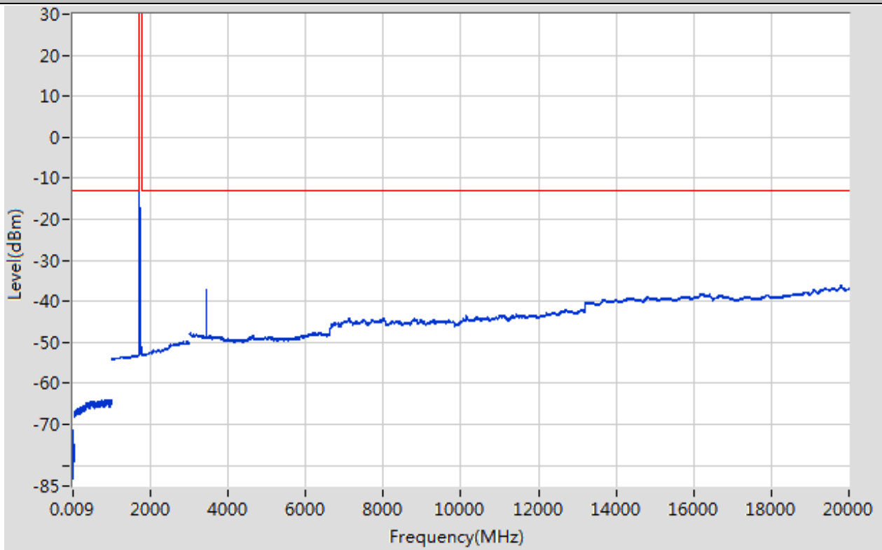
Band66_20MHz_16QAM_132072_1RB#50
