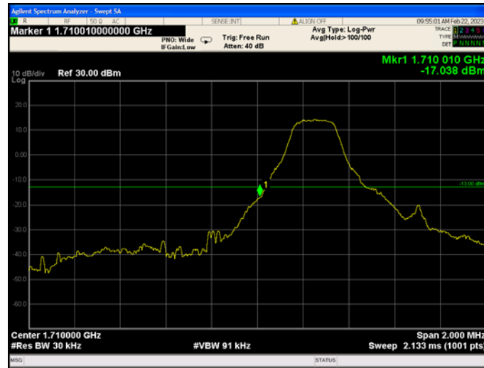
Band4-1.4MHz-QPSK-19957-1RB#5
