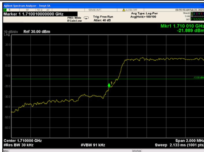
Band4-1.4MHz-QPSK-19957-6RB#0
