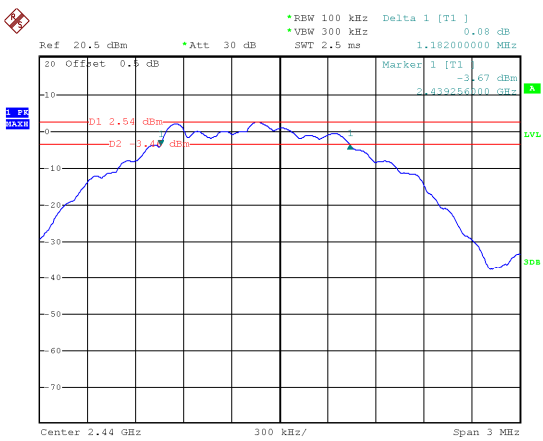
Mode: TX GFSK 2M channel 19
