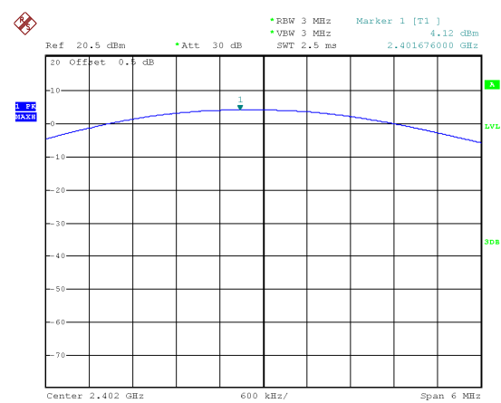
Mode: TX GFSK 1M channel 0
