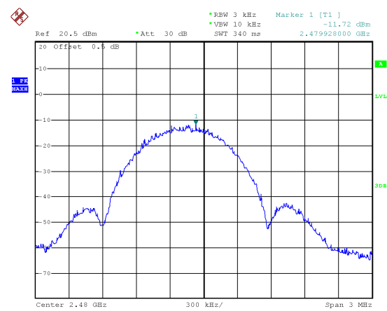
Mode: TX GFSK 1M channel 39
