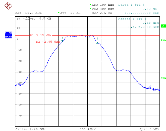
Mode: TX GFSK 1M channel 39
