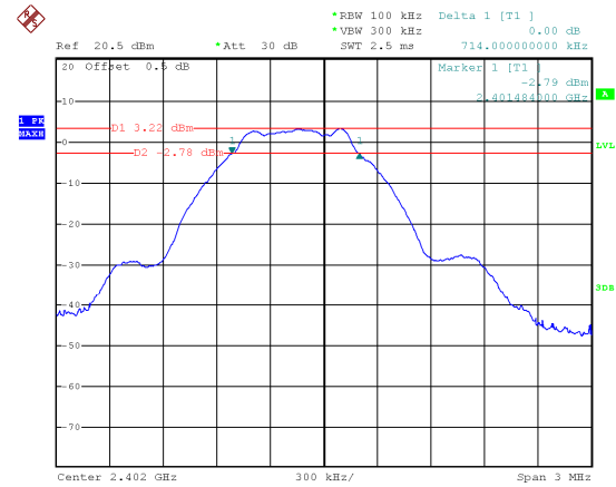
Mode: TX GFSK 1M channel 0
