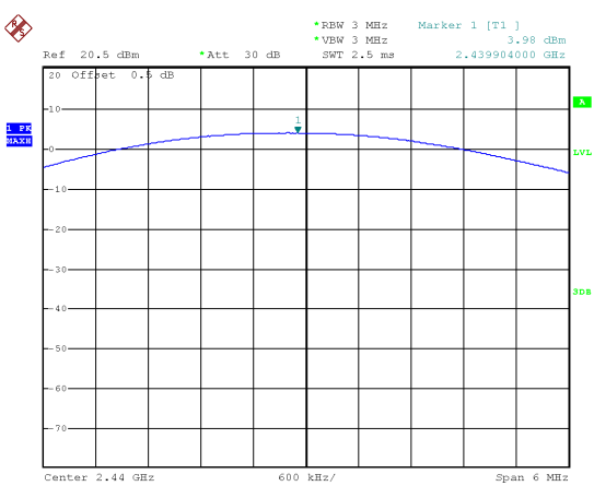
Mode: TX GFSK 1M channel 19
