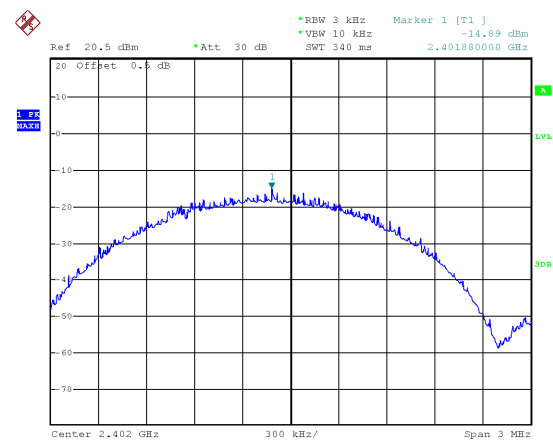
Mode: TX GFSK 2M channel 0
