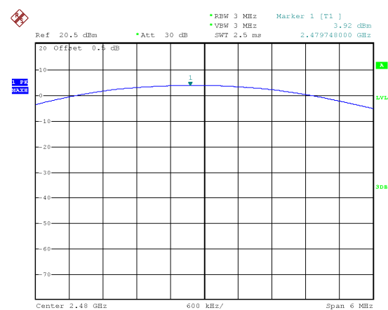
Mode: TX GFSK 2M channel 39
