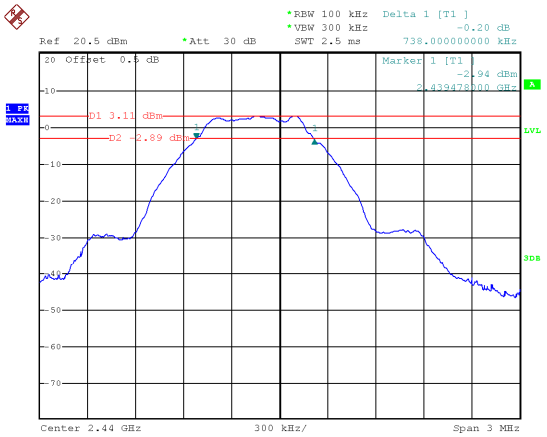
Mode: TX GFSK 1M channel 19
