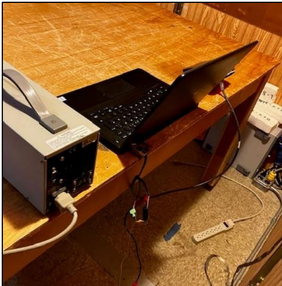
Photograph 7: Conducted Emissions (Back)
