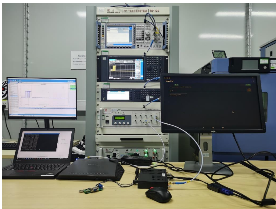
Photograph 3: Set-up photo for DFS
