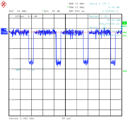
NTNV-11G-Ant1-2462
