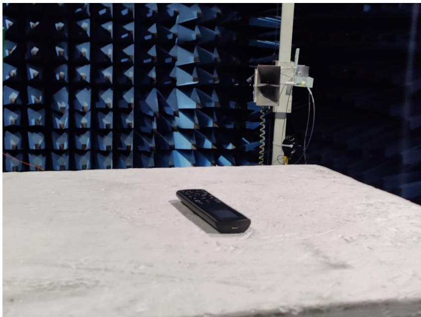
Radiated Spurious Emissions Above 1GHz
