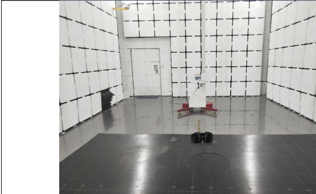
Band edge emissions (Radiated) Emissions in restricted frequency bands (below 1GHz)
