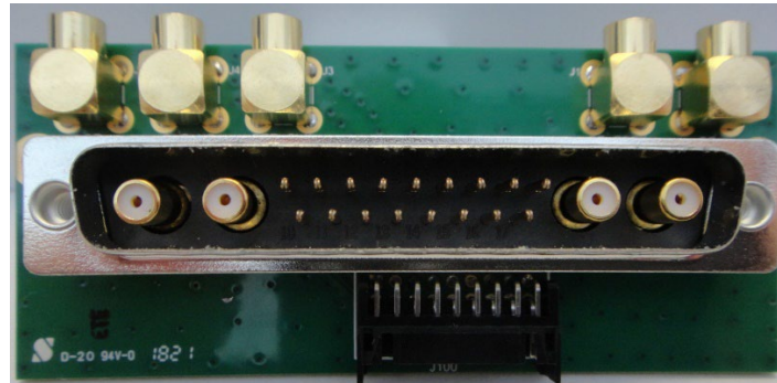
Figure 11: 031-00378 Digital Interface PCB Assembly Top view
