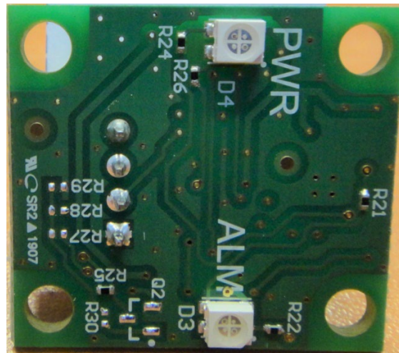
Figure 10: 031-00282 LED Power Alarm PCB Assembly Bottom view
