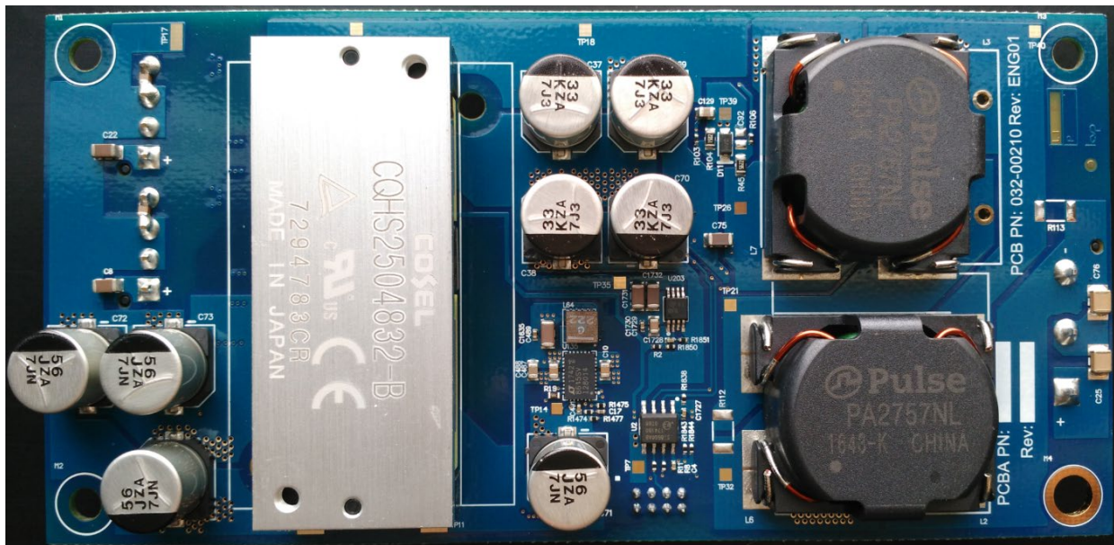
Figure 13: 031-00296 32VDC Public Safety Power Supply PCB Assembly Top view
