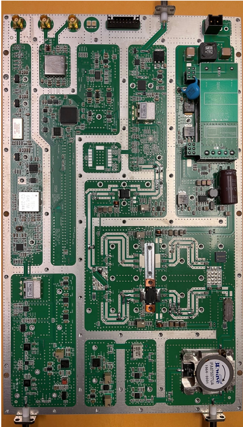
Figure 5: RF Public Safety 700MHz PCB Assembly Top View
