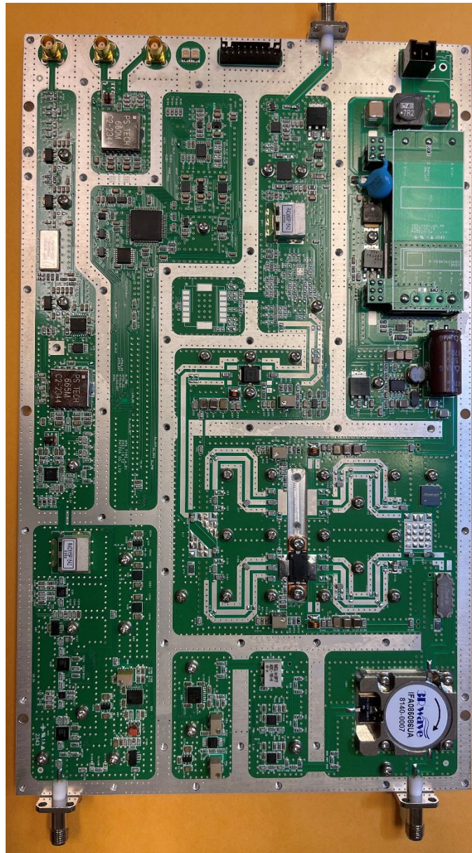
Figure 7: RF Public Safety 800MHz PCB Assembly Top View
