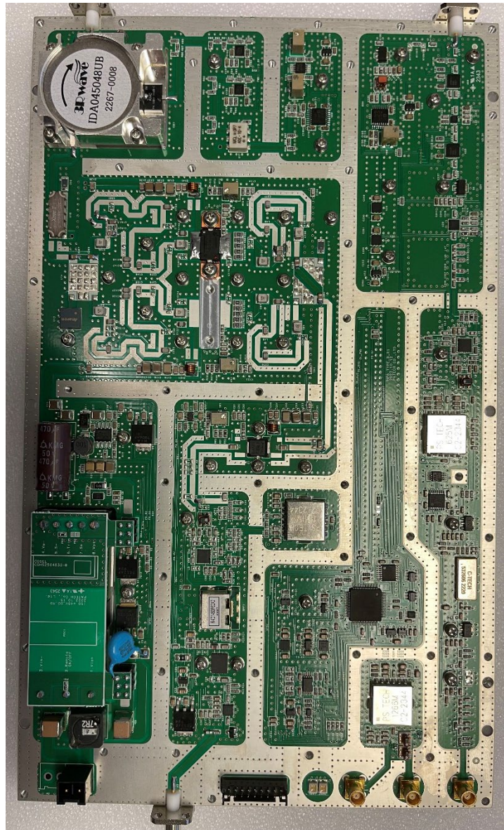
Figure 3: RF Public Safety 450MHz PCB Assembly Top View
