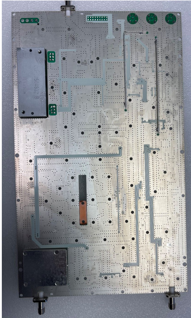
Figure 2: RF Public Safety 415MHz PCB Assembly Bottom View
