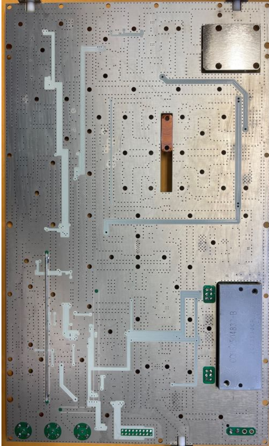
Figure 6: RF Public Safety 700MHz PCB Assembly Bottom View
