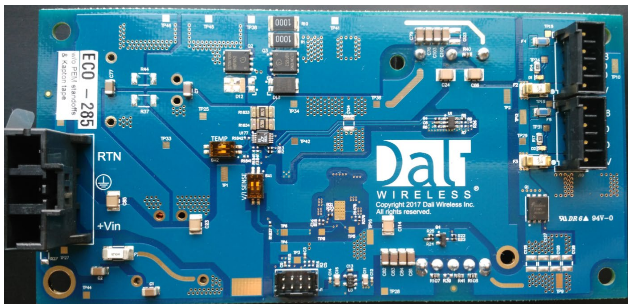
Figure 14: 031-00296 32VDC Public Safety Power Supply PCB Assembly Bottom view
