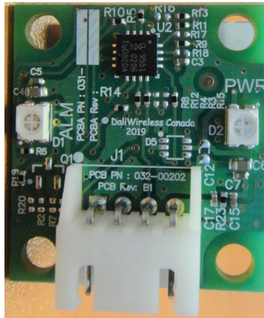
Figure 9: 031-00282 LED Power Alarm PCB Assembly Top view
