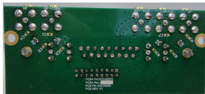
Figure 12: 031-00378 Digital Interface PCB Assembly Bottom view
