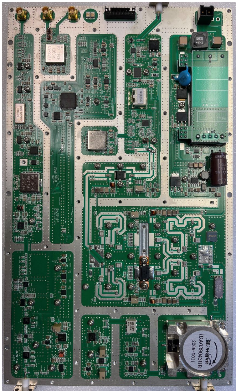
Figure 1: RF Public Safety 415MHz PCB Assembly Top View
