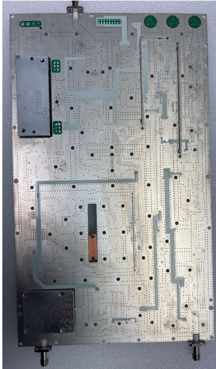
Figure 4: RF Public Safety 450MHz PCB Assembly Bottom View
