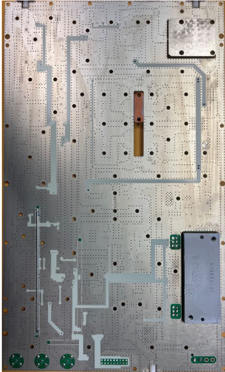
Figure 8: RF Public Safety 800MHz PCB Assembly Bottom View
