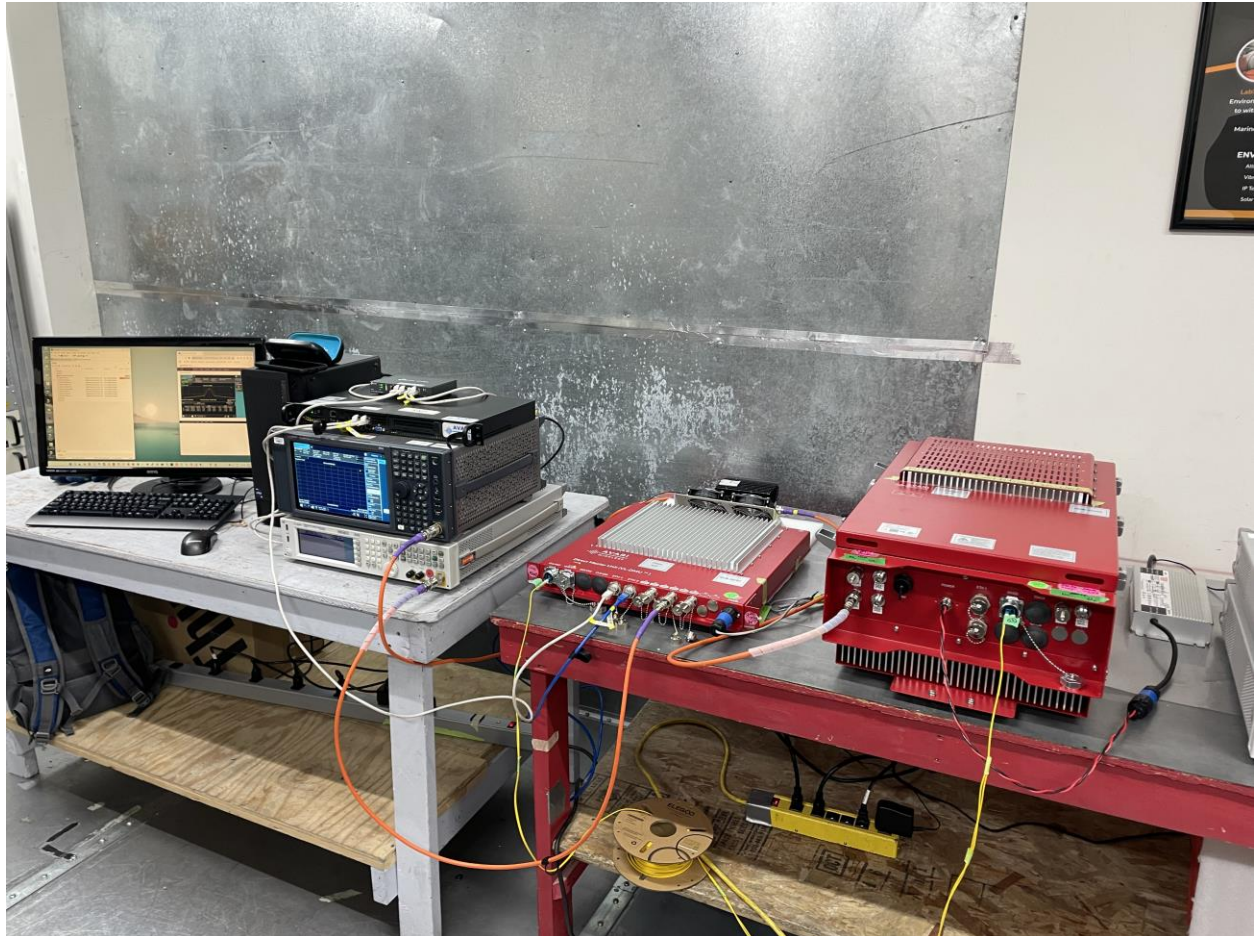
Figure 1: Test Station
