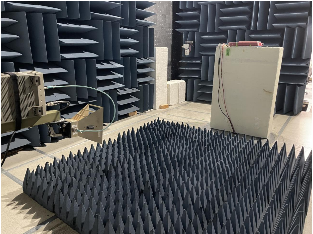
Figure 4: Radiated Emissions (Above 1GHz) Emissions Test Setup
