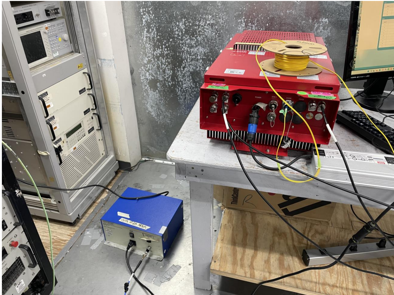
Figure 5: Conducted Emission Test Setup – EUT
