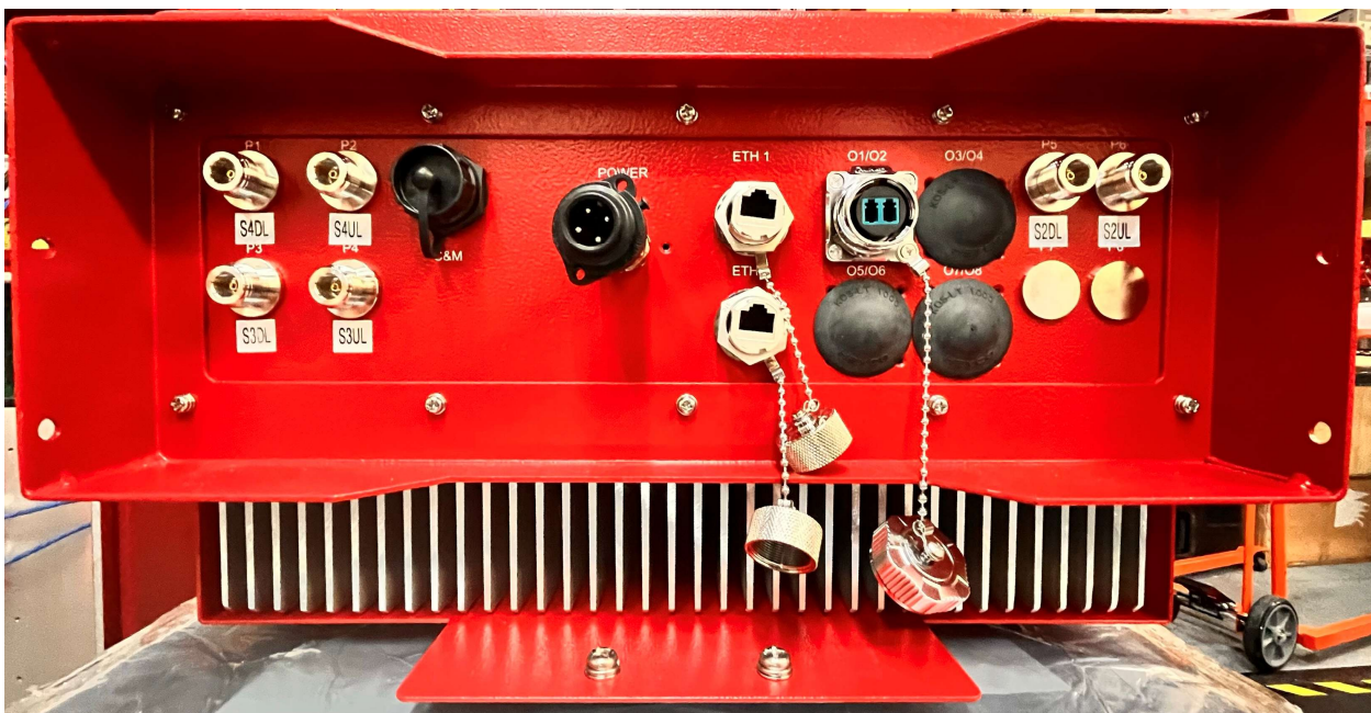
Figure 5: Connector panel view
