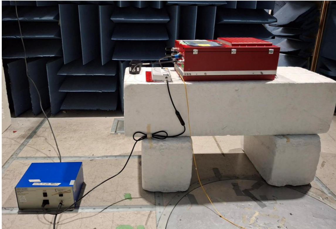
Figure 3: Conducted Emission Test Setup – EUT
