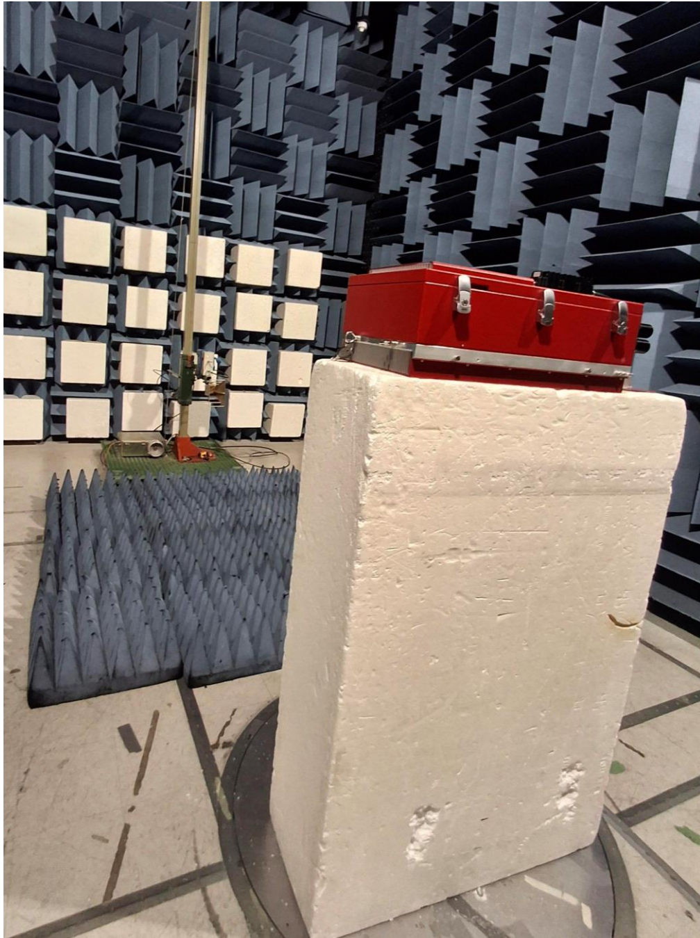
Figure 2: Radiated Emissions (Above 1GHz) Emissions Test Setup
