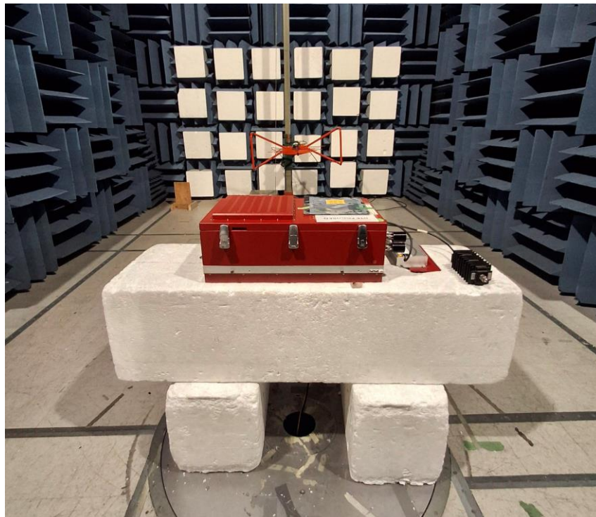
Figure 2: Radiated Emissions Test Setup (30 MHz – 1 GHz)
