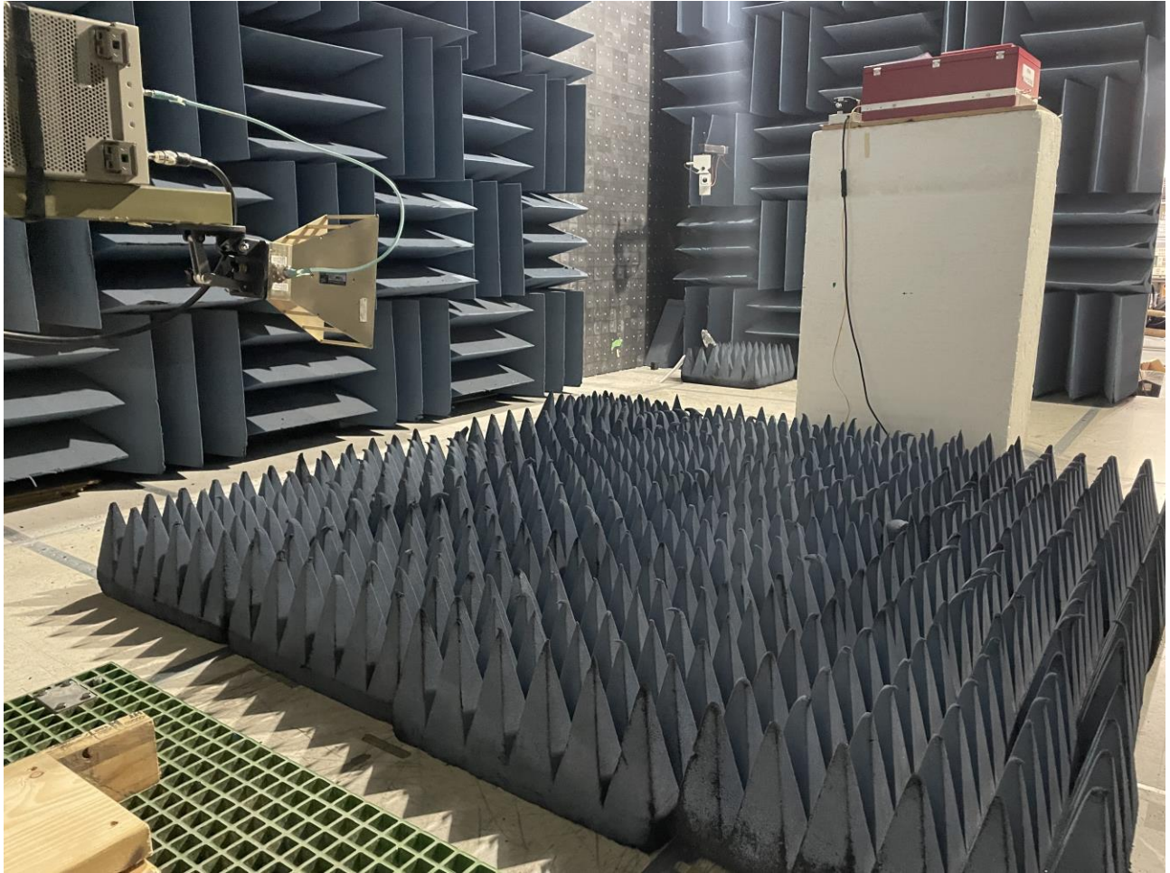
Figure 4: Test setup for radiated emissions above 1000 MHz
