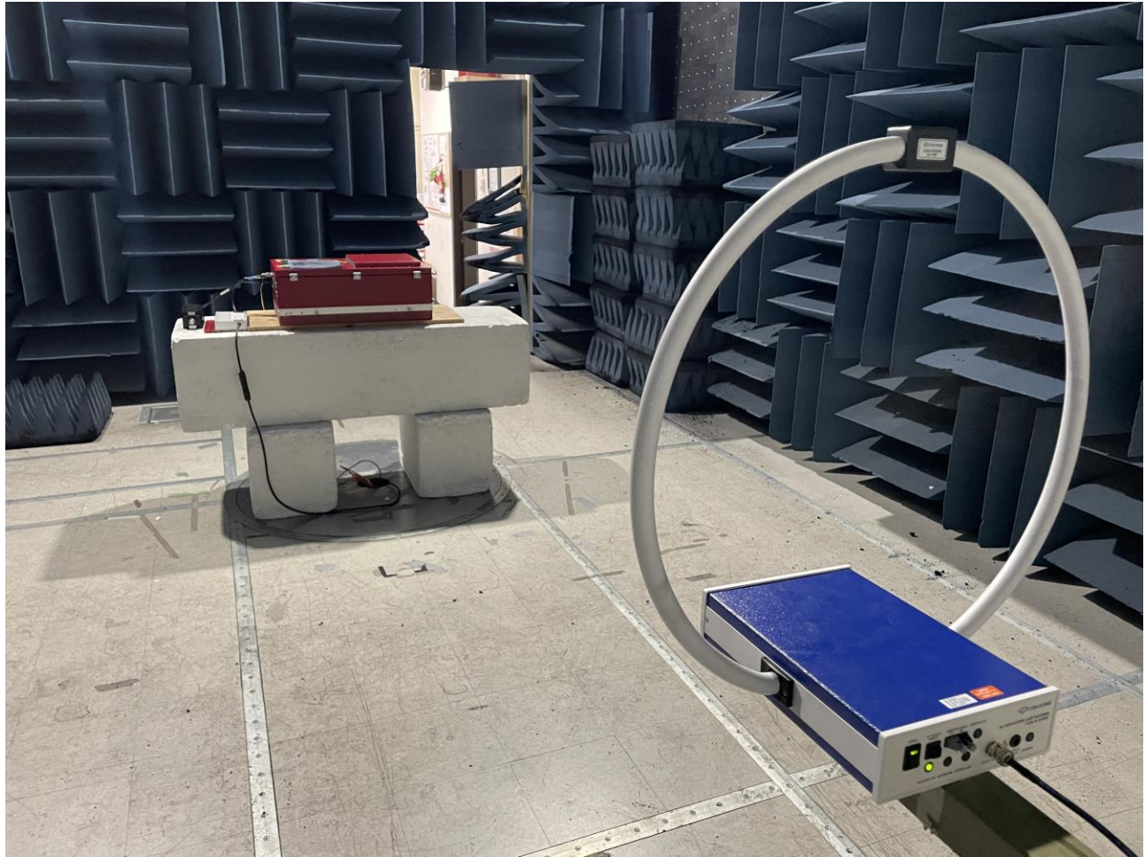
Figure 2: Test setup for radiated emissions below 30 MHz
