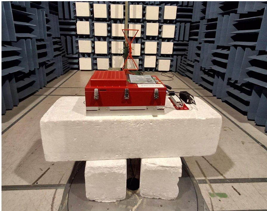
Figure 2: Radiated Emissions Test Setup (30 MHz – 1 GHz)
