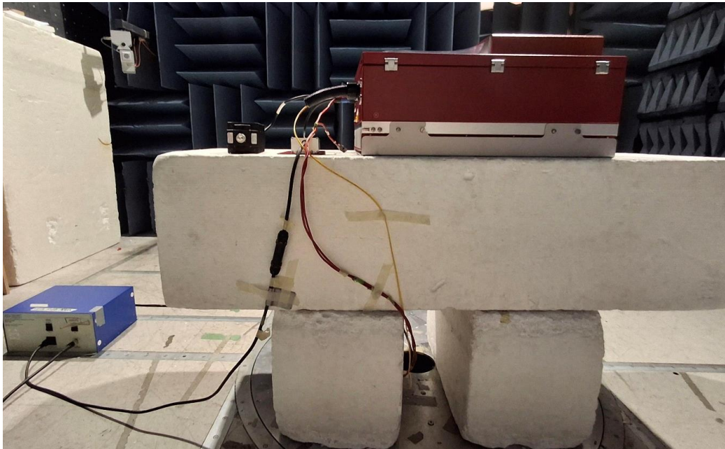
Figure 3: Conducted Emission Test Setup – EUT
