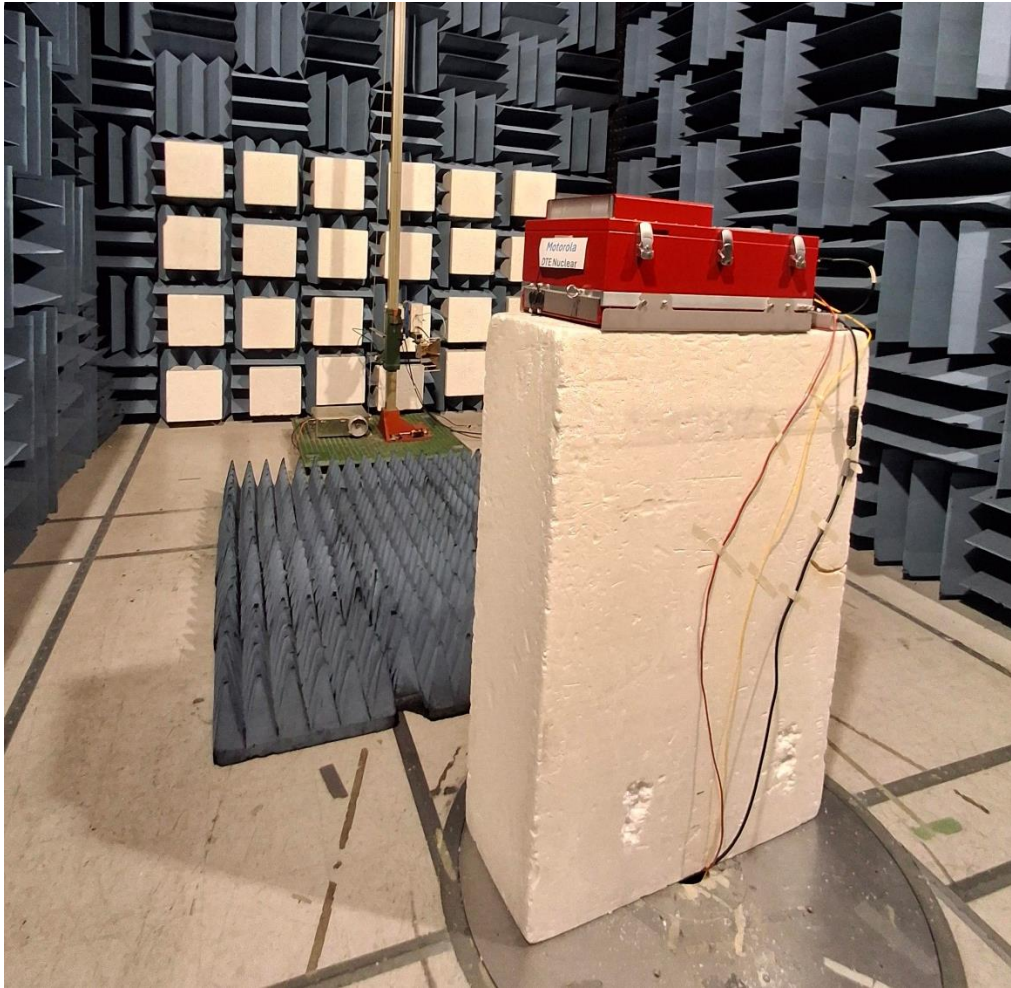
Figure 2: Radiated Emissions (Above 1GHz) Emissions Test Setup
