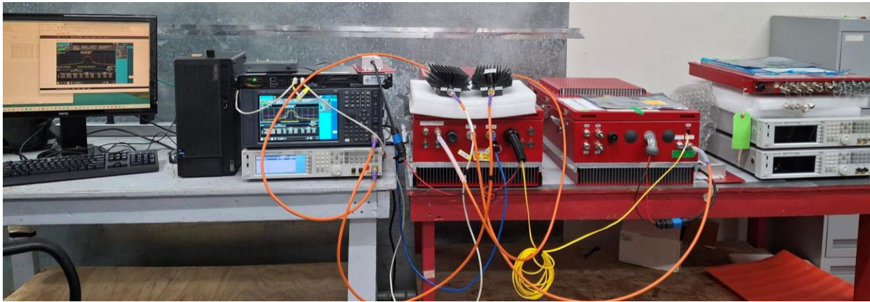
Figure 1: Test Station
