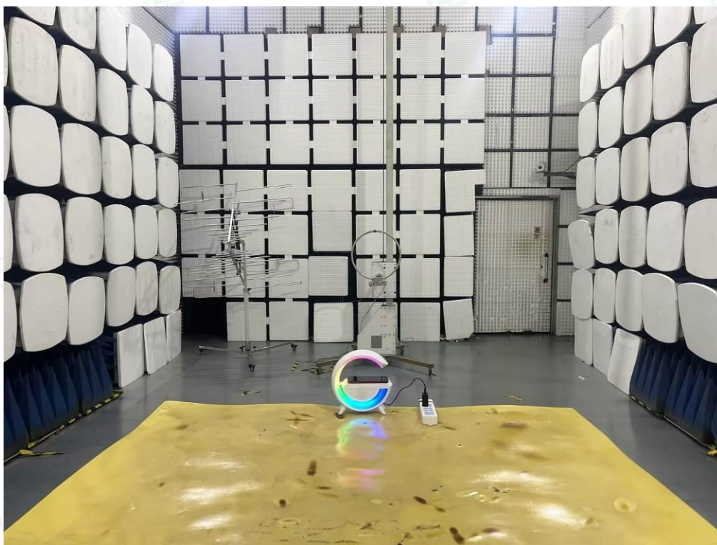
Below 30MHz
