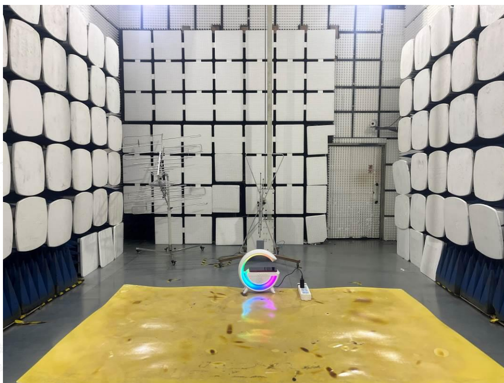
Below 1GHz
