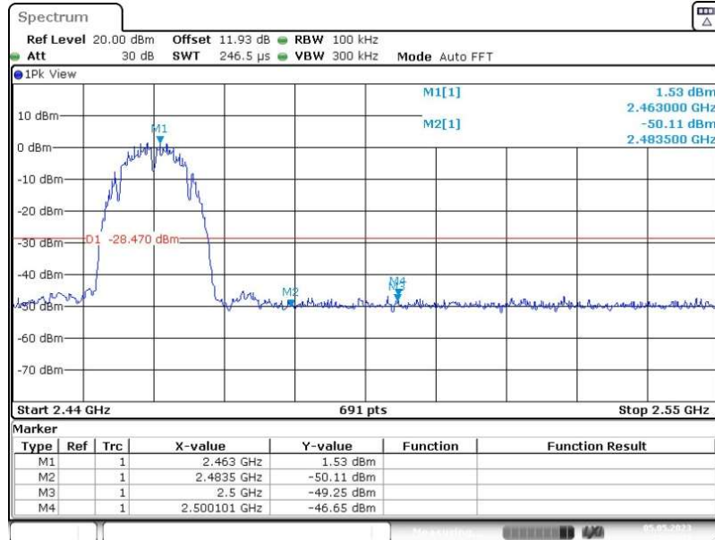
11B_Ant1_High_2462
