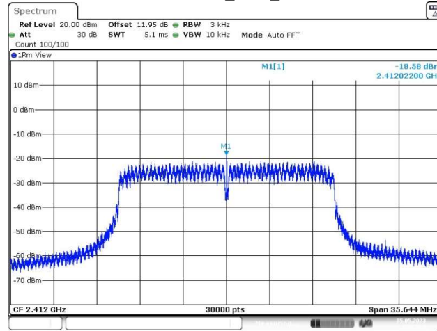
11N20SISO_Ant1_2412
