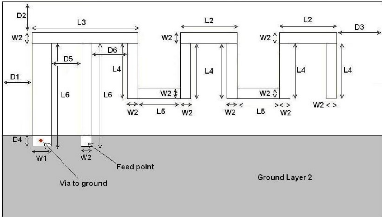
Figure 1: Antenna Dimensions
