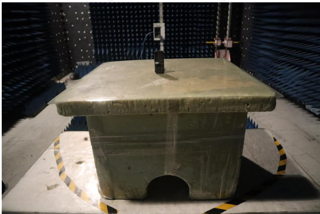
RE (Above 1GHz)
