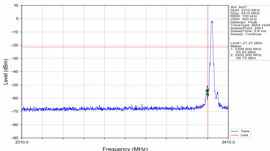
1M_LCH_2402MHz_Ant1_NTNV
