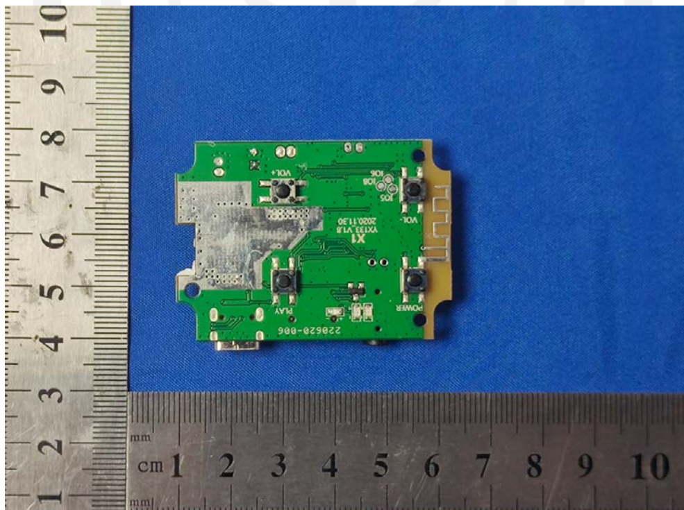
Antenna Location
