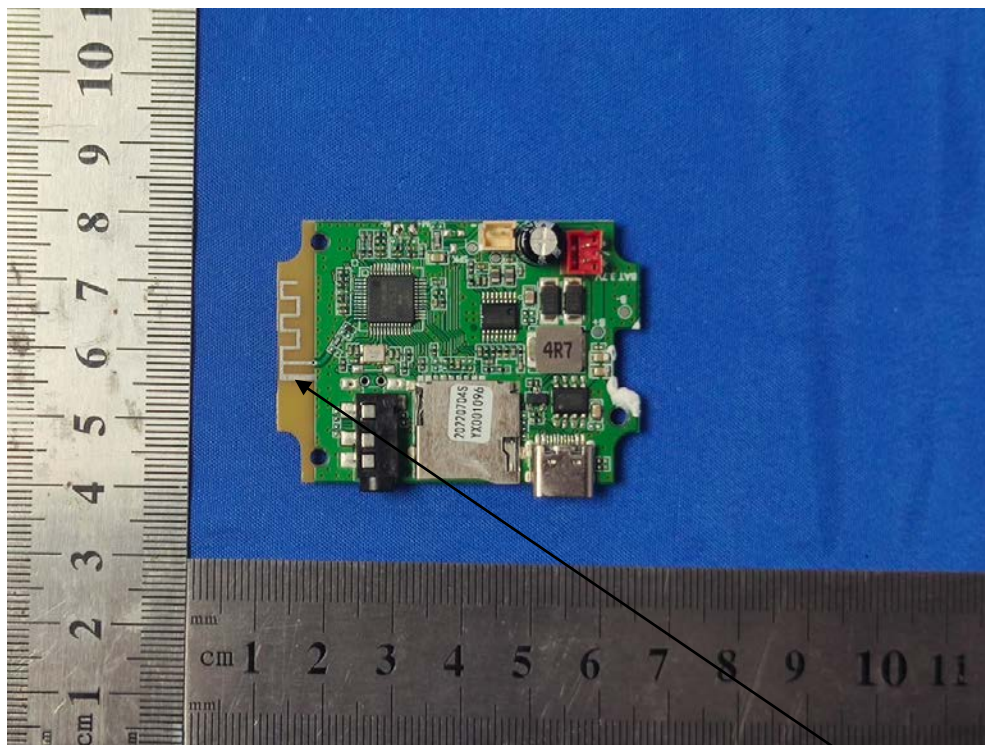
Antenna Location
