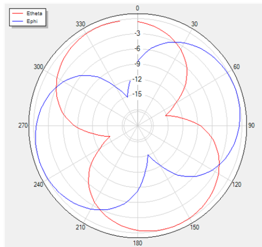
H Theta=0 freq=2400MHz
