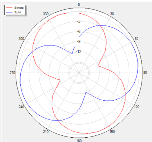
H Theta=0 freq=2450MHz
