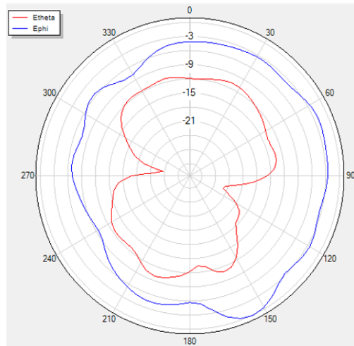
V Phi=90 freq=2400MHz
