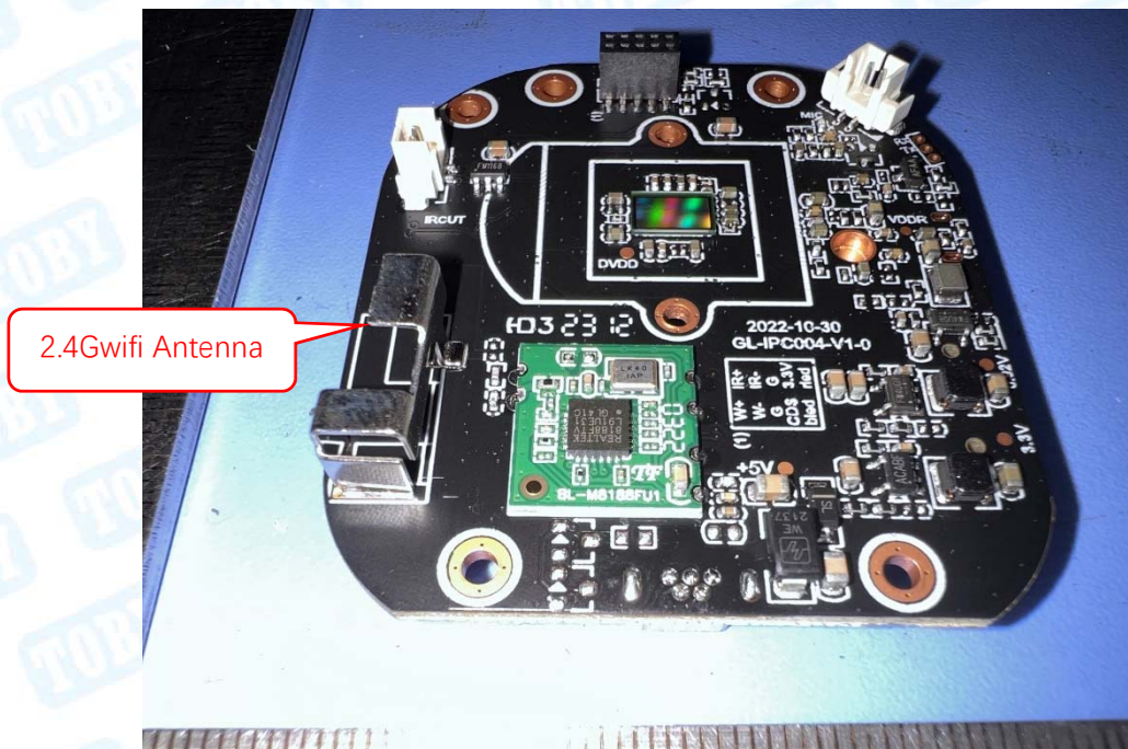
Photo 10 Appearance of PCB
