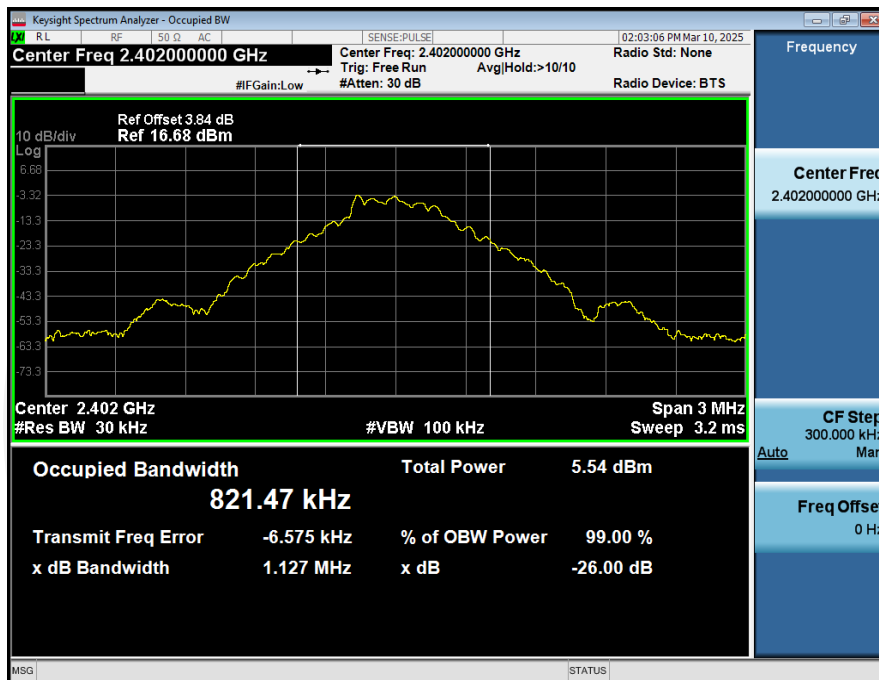
99%_Occupied_Bandwidth_NVNT_ANT1_1-DH1_2402_00
