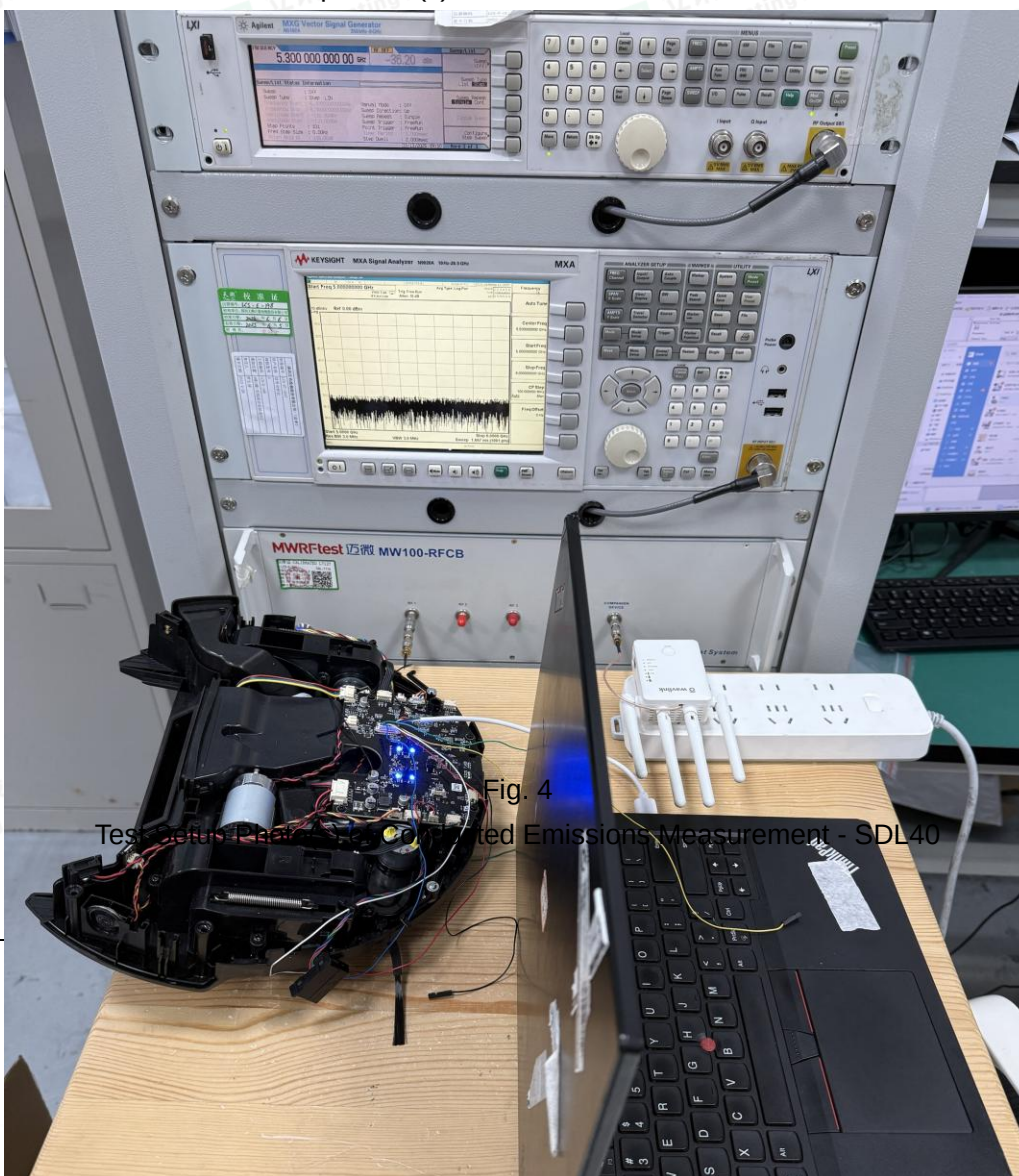
Test Setup Photo(s) of DFS Measurement - - SL40
