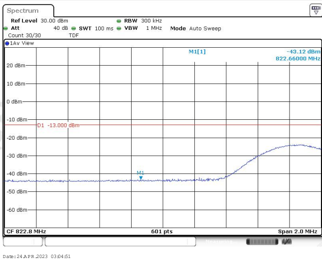
Band26-15MHz-16QAM-26853-75RB#0
