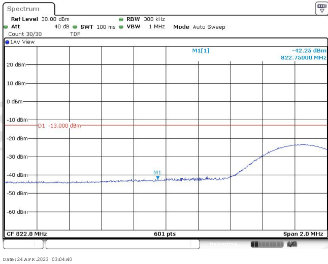
Band26-15MHz-QPSK-26853-75RB#0
