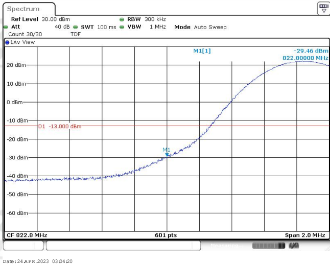
Band26-15MHz-QPSK-26853-1RB#74
