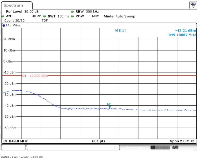
Band26-15MHz-QPSK-26965-1RB#74
