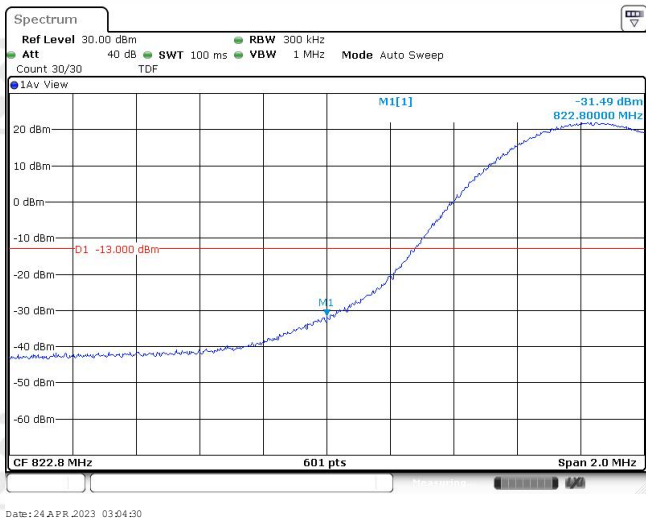
Band26-15MHz-16QAM-26853-1RB#74
