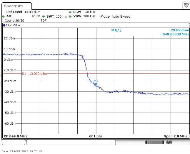
Band26-3MHz-16QAM-26793-1RB#0
