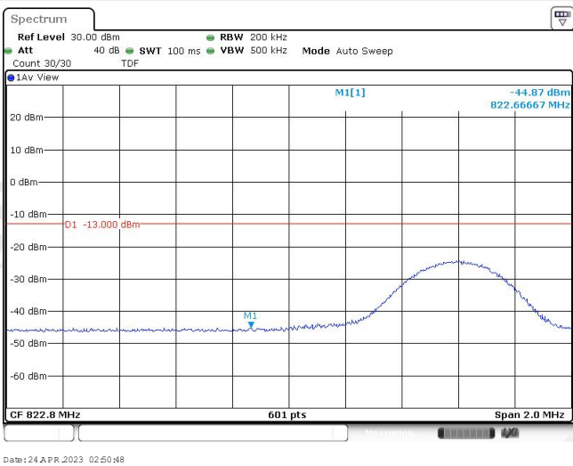
Band26-10MHz-16QAM-26828-50RB#0
