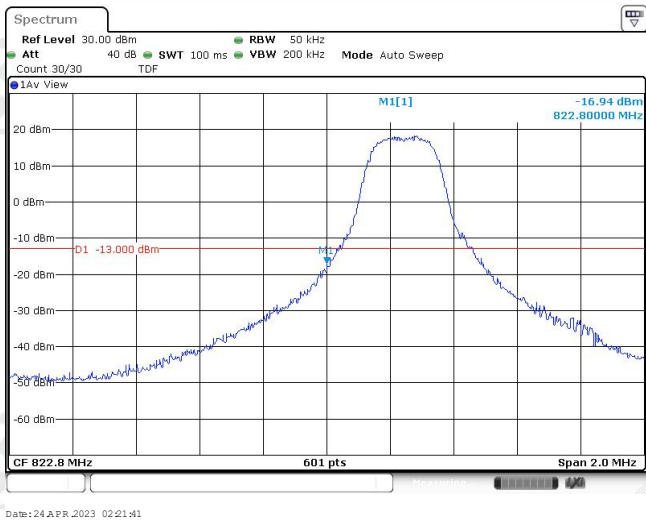
Band26-3MHz-16QAM-26793-1RB#14
