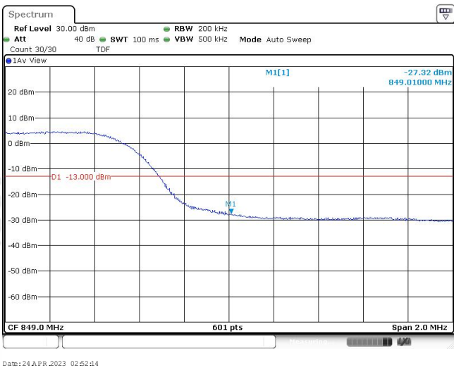
Band26-10MHz-16QAM-26828-1RB#0
