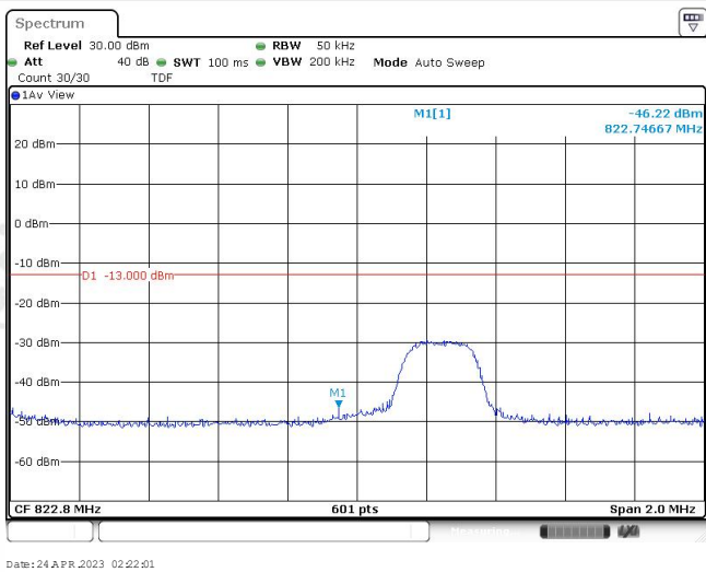
Band26-3MHz-16QAM-26793-15RB#0
