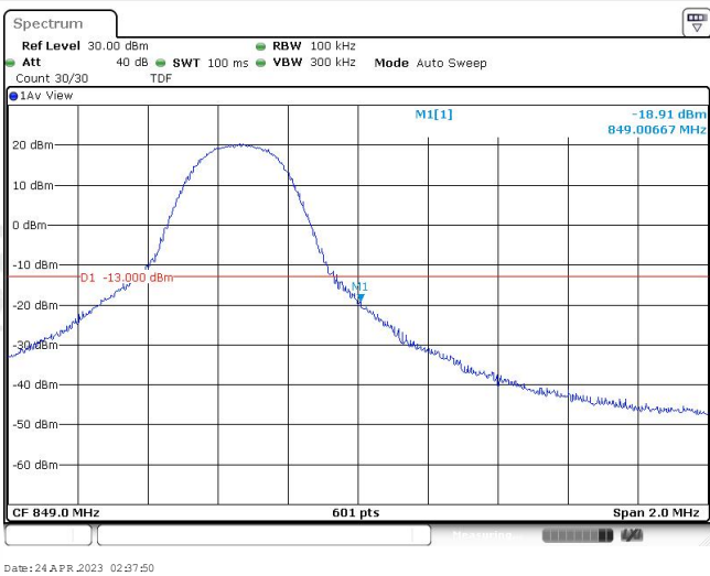
Band26-5MHz-QPSK-27015-25RB#0
