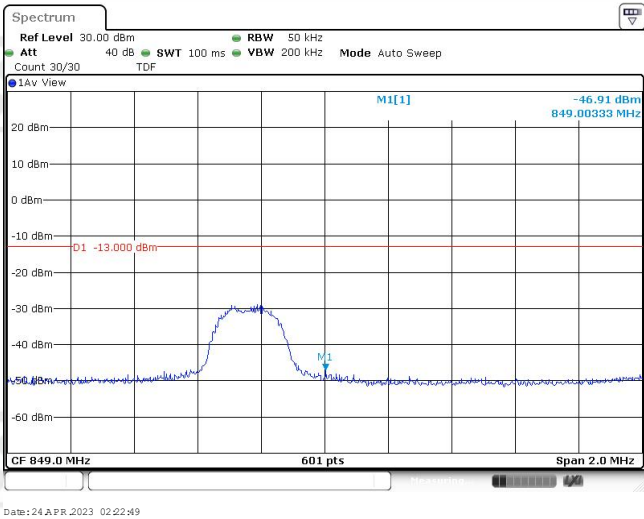
Band26-3MHz-16QAM-27025-1RB#14
