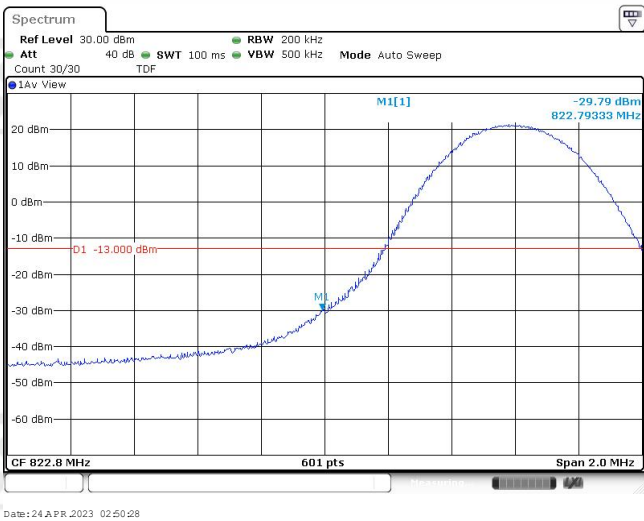
Band26-10MHz-16QAM-26828-1RB#49
