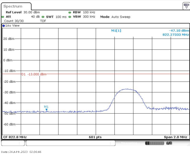
Band26-5MHz-16QAM-26803-25RB#0
