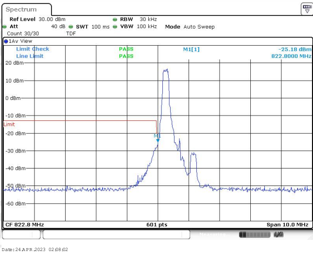
Band26-1.4MHz-16QAM-26785-1RB#5
