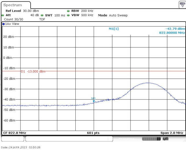
Band26-10MHz-QPSK-26828-50RB#0
