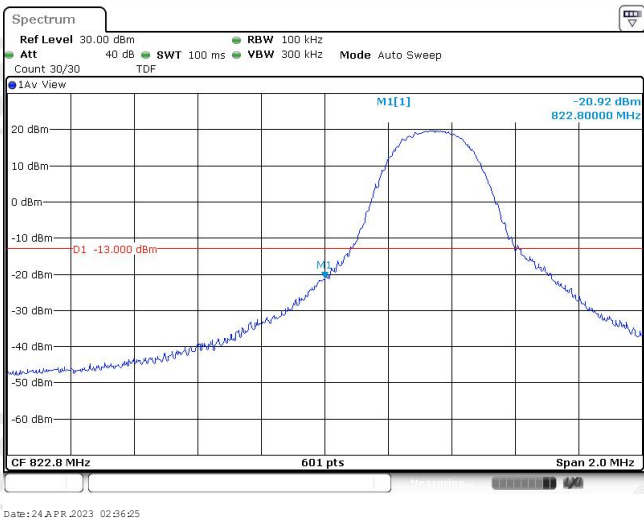
Band26-5MHz-16QAM-26803-1RB#24
