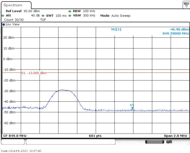
Band26-5MHz-16QAM-27015-1RB#24
