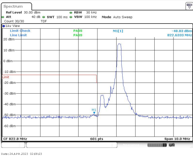
Band26-1.4MHz-16QAM-26785-6RB#0
