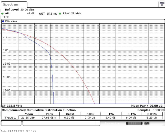
Band26-1.4MHz-16QAM-26785-6RB#0
