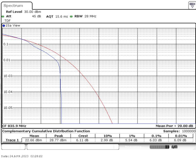
Band26-3MHz-16QAM-26909-15RB#0
