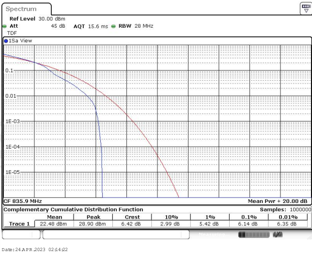
Band26-1.4MHz-16QAM-26909-6RB#0
