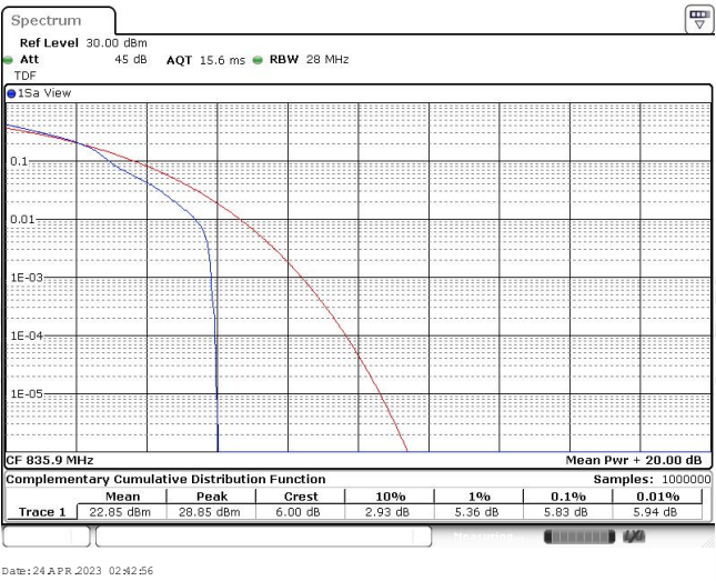
Band26-5MHz-16QAM-26909-25RB#0
