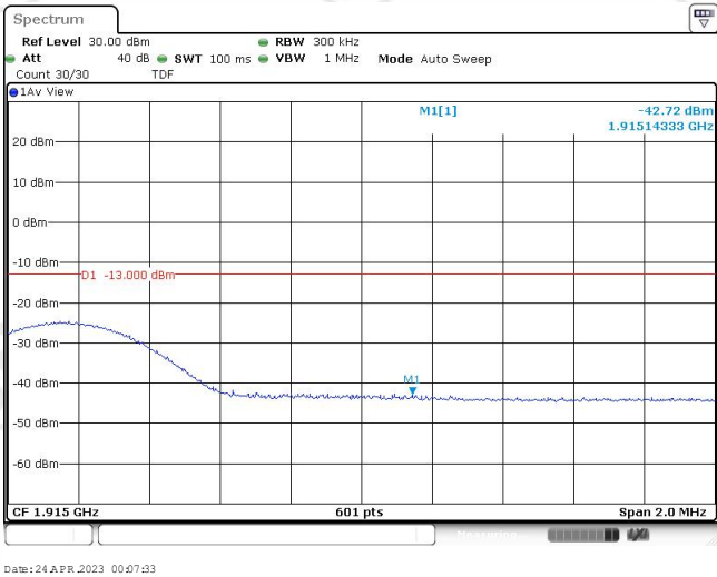
Band25-15MHz-16QAM-26615-1RB#74
