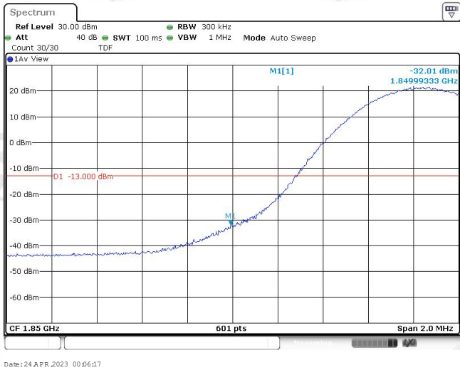
Band25-15MHz-16QAM-26115-1RB#74
