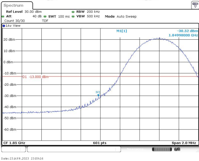
Band25-10MHz-16QAM-26090-1RB#49
