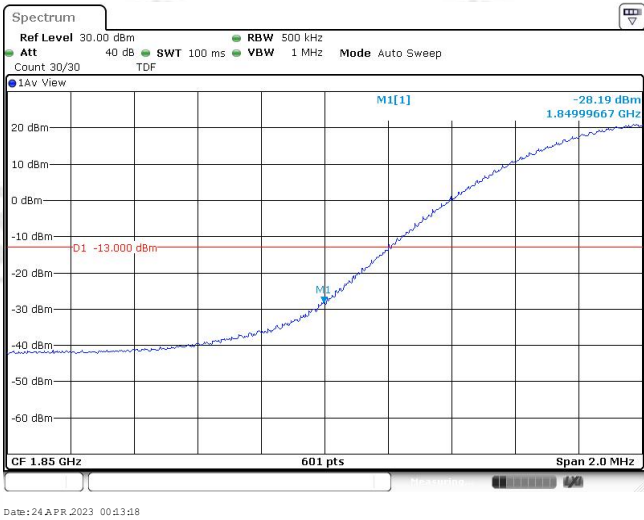
Band25-20MHz-16QAM-26140-1RB#99
