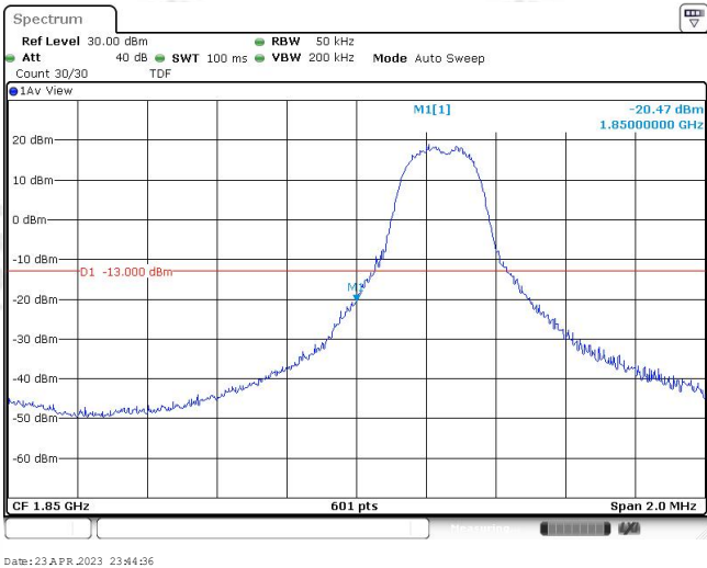
Band25-3MHz-16QAM-26055-1RB#14
