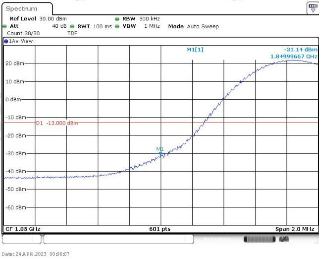
Band25-15MHz-QPSK-26115-1RB#74
