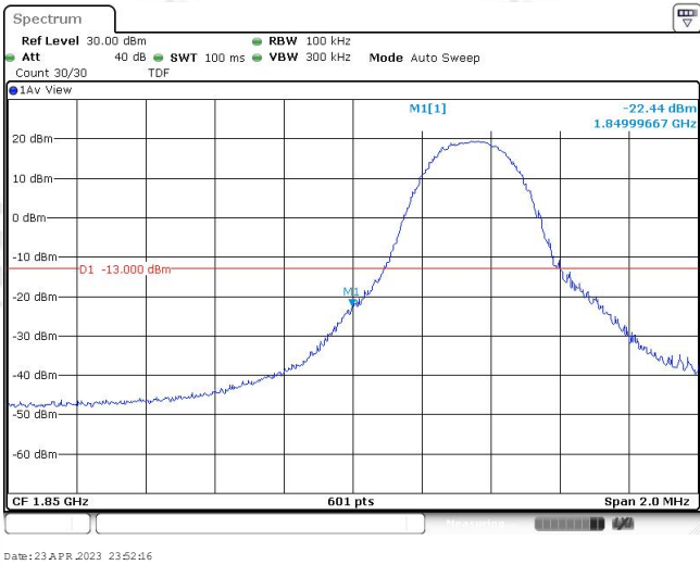
Band25-5MHz-16QAM-26065-1RB#24
