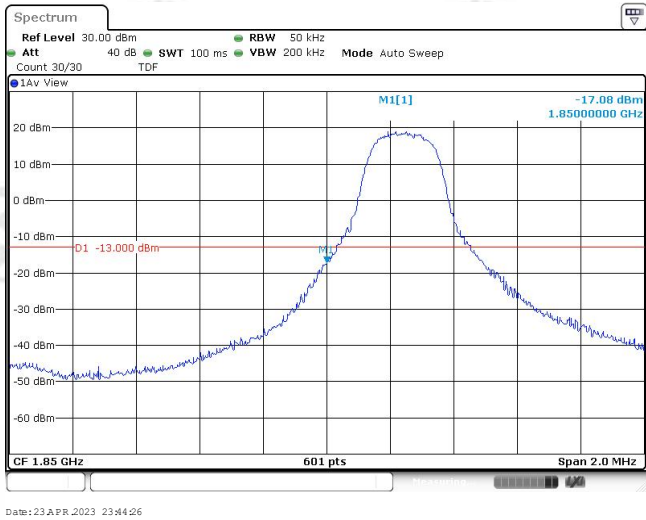
Band25-3MHz-QPSK-26055-1RB#14
