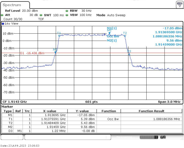
Band25-1.4MHz-16QAM-26047-6RB#0-1.088
