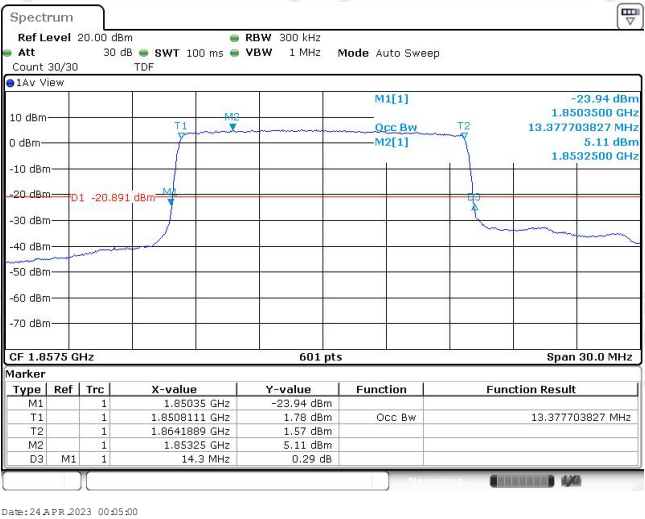
Band25-15MHz-16QAM-26365-75RB#0-13.428
