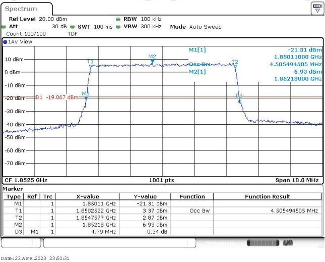
Band25-5MHz-16QAM-26365-25RB#0-4.505
