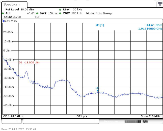
Band25-1.4MHz-QPSK-26683-1RB#5
