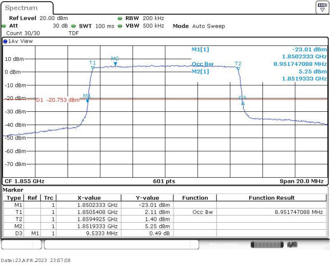
Band25-10MHz-16QAM-26365-50RB#0-8.952
