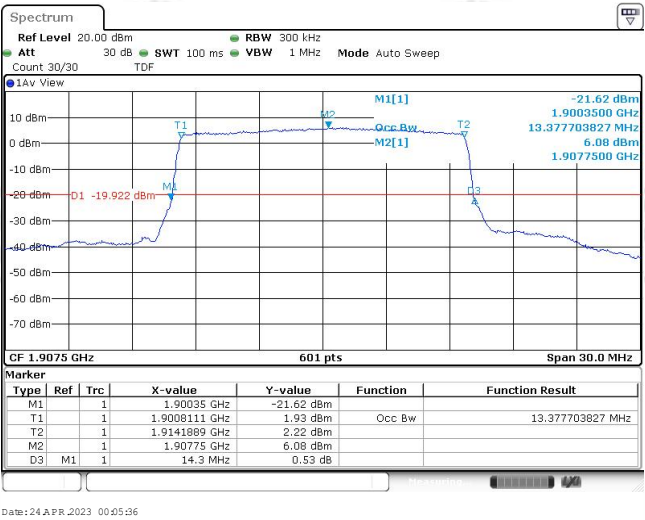
Band25-15MHz-16QAM-26115-75RB#0-13.378
