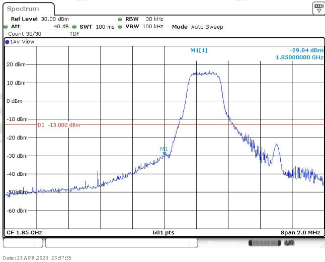
Band25-1.4MHz-16QAM-26047-1RB#5
