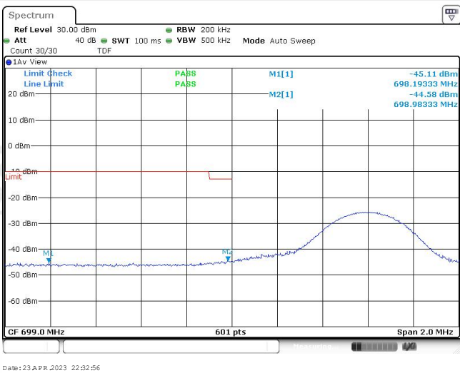
Band12-10MHz-QPSK-23060-50RB#0
