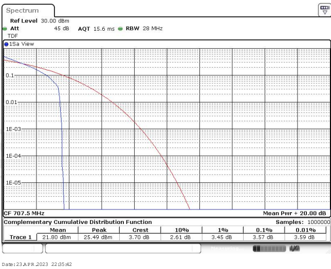
Band12-10MHz-QPSK-23095-50RB#0
