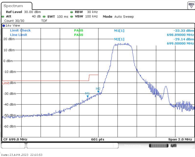
Band12-1.4MHz-16QAM-23017-1RB#5
