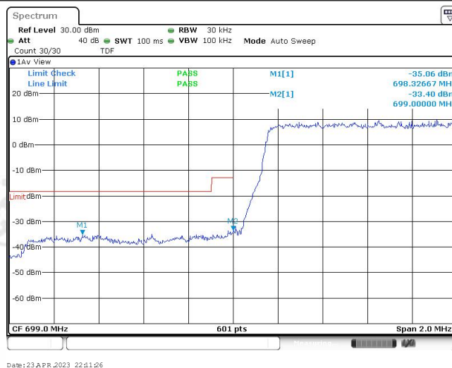
Band12-1.4MHz-QPSK-23173-1RB#0
