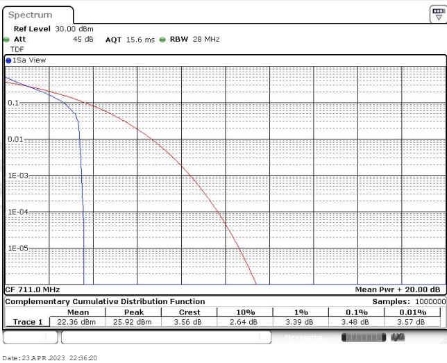
Band12-10MHz-QPSK-23130-50RB#0
