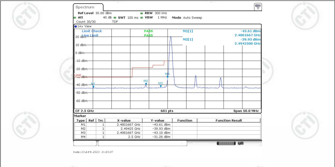
Band7-15MHz-16QAM-20825-1RB#74
