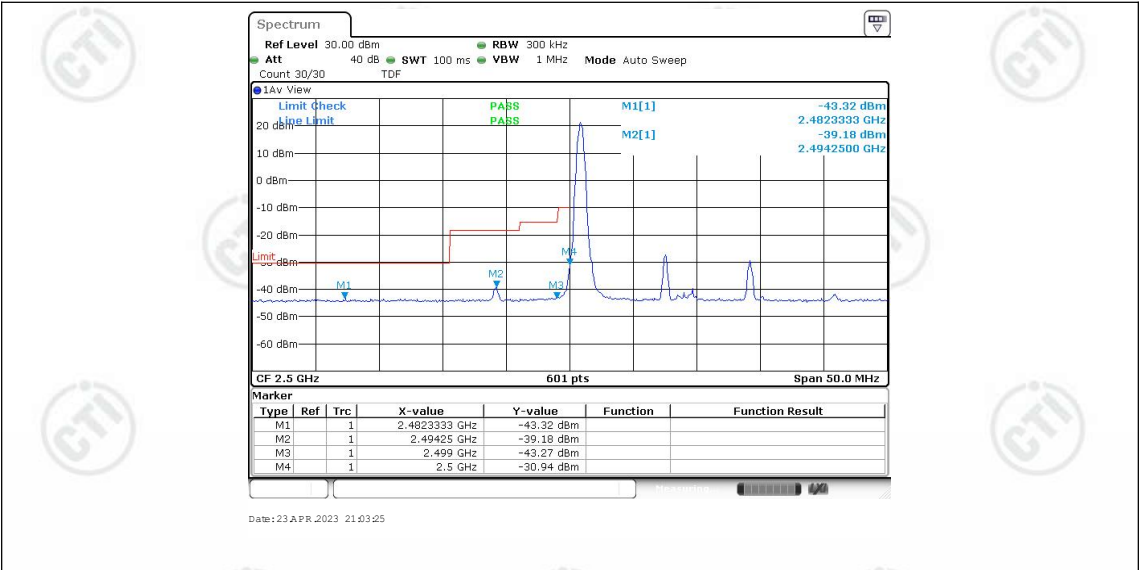
Band7-15MHz-QPSK-20825-1RB#74
