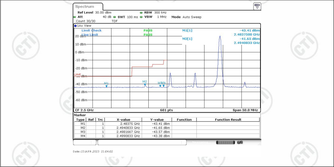
Band7-15MHz-16QAM-20825-75RB#0
