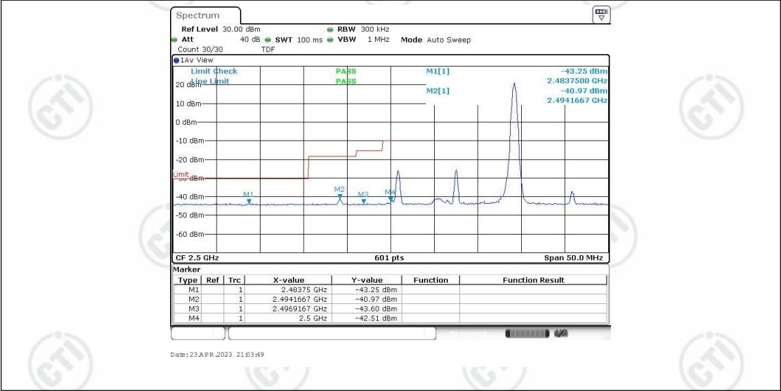
Band7-15MHz-QPSK-20825-75RB#0
