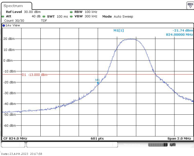
Band5-5MHz-16QAM-20425-1RB#24
