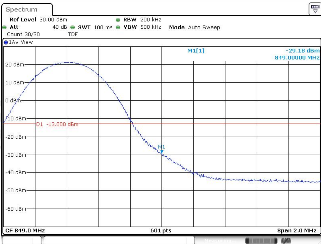
Band5-10MHz-QPSK-20600-1RB#49
