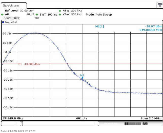
Band5-10MHz-16QAM-20600-50RB#0
