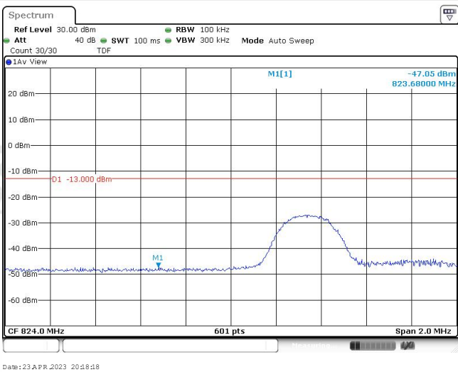
Band5-5MHz-16QAM-20425-25RB#0
