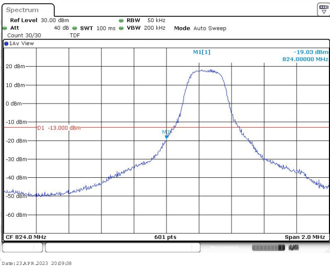
Band5-3MHz-16QAM-20415-1RB#14
