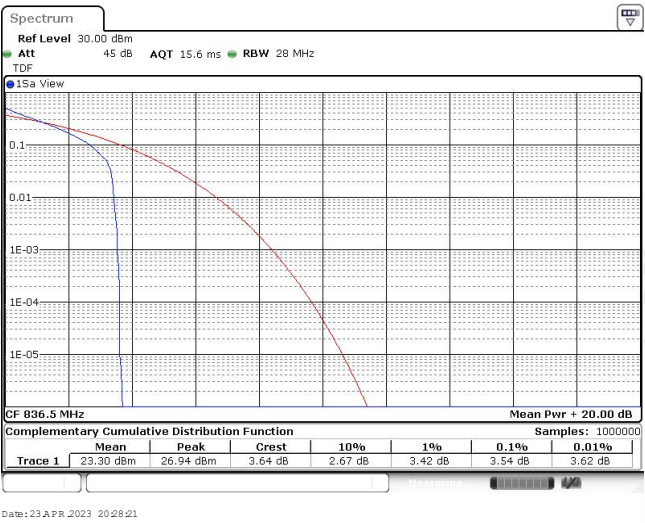
Band5-10MHz-QPSK-20525-50RB#0
