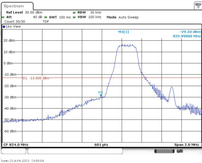
Band5-1.4MHz-16QAM-20407-1RB#5
