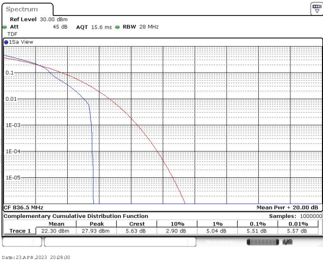
Band5-10MHz-16QAM-20525-50RB#0
