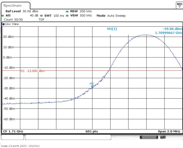
Band4-10MHz-QPSK-20000-1RB#49
