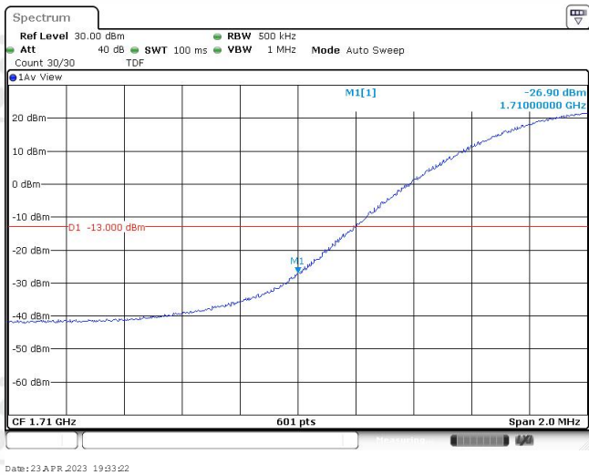
Band4-20MHz-16QAM-20050-1RB#99
