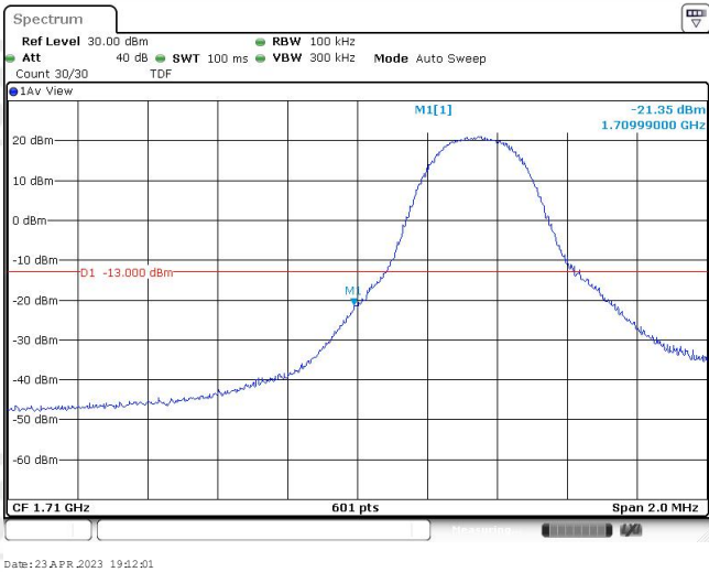
Band4-5MHz-QPSK-19975-1RB#24
