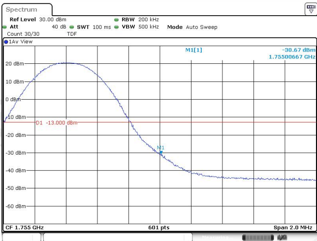
Band4-10MHz-QPSK-20350-1RB#49
