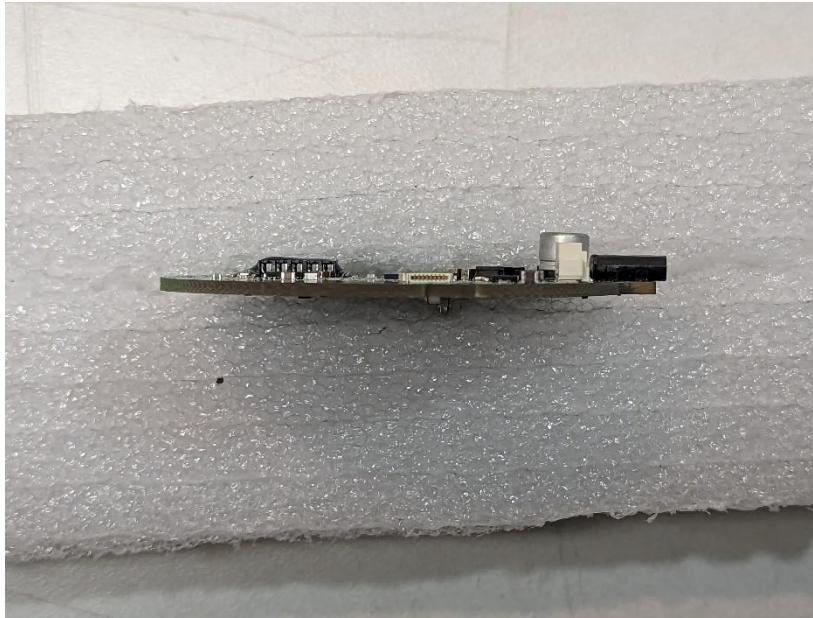
Photograph 21: Side 1 View of PCB Removed from Enclosure
