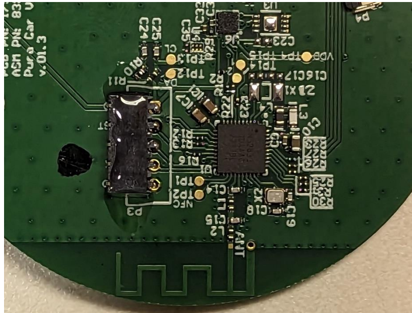
Photograph 17: Closeup View of RF Circuitry on Top of PCB
