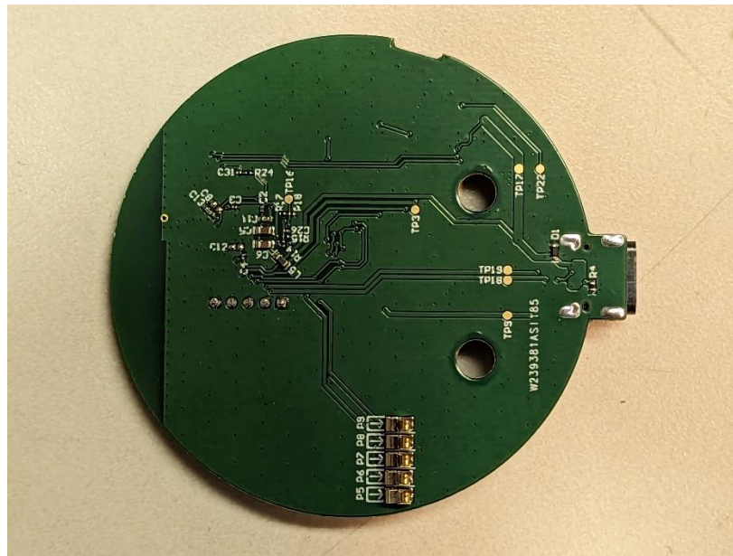
Photograph 16: Bottom View of PCB Removed from Enclosure
