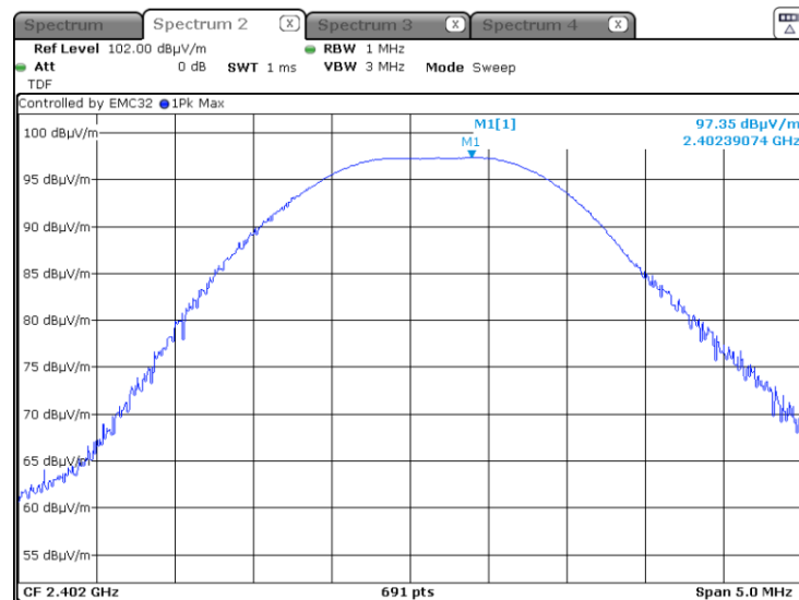
Graph 4: Lowest Channel Output Power Plot
