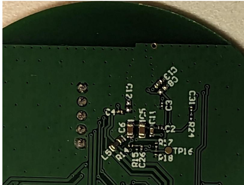
Photograph 18: Closeup View of RF Circuitry on Bottom of PCB
