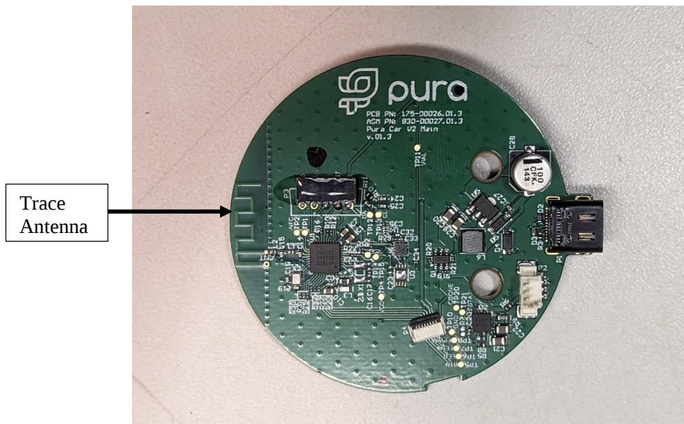
Photograph 15: Top View of PCB Removed from Enclosure and Trace Antenna
