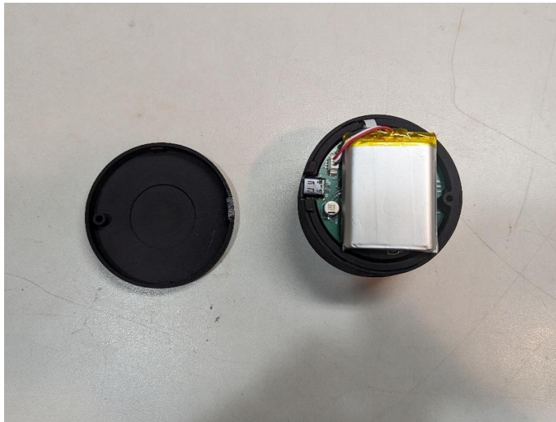
Photograph 13: View of EUT with Bottom Cover Removed Showing How PCB Fits in Enclosure with Battery
