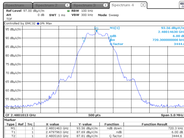
Graph 3: Highest Channel Bandwidth
