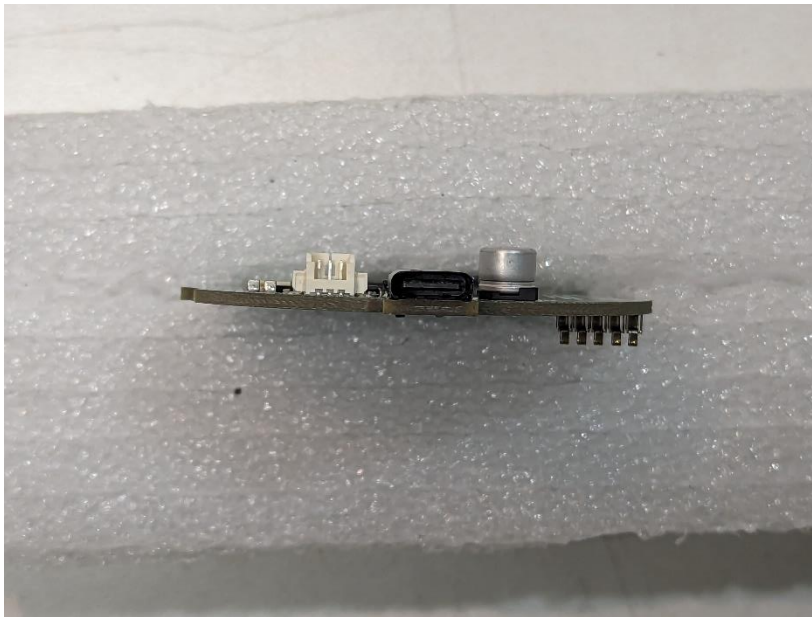
Photograph 20: Back View of PCB Removed from Enclosure
