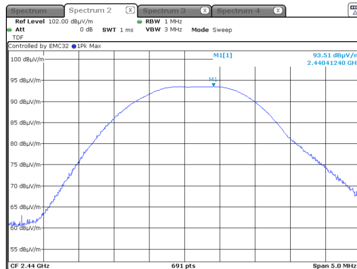
Graph 5: Middle Channel Output Power
