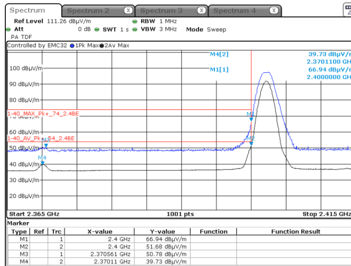
Graph 7: Radiated Lower Band Edge Plot
