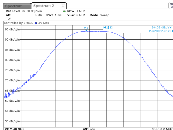
Graph 6: Highest Channel Output Power Plot
