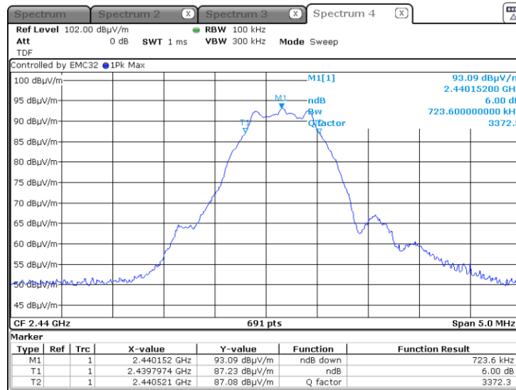
Graph 2: Middle Channel Bandwidth
