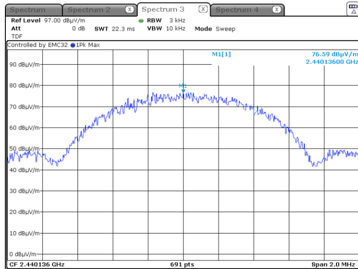
Graph 10: Middle Channel 3 kHz PSD Plot
