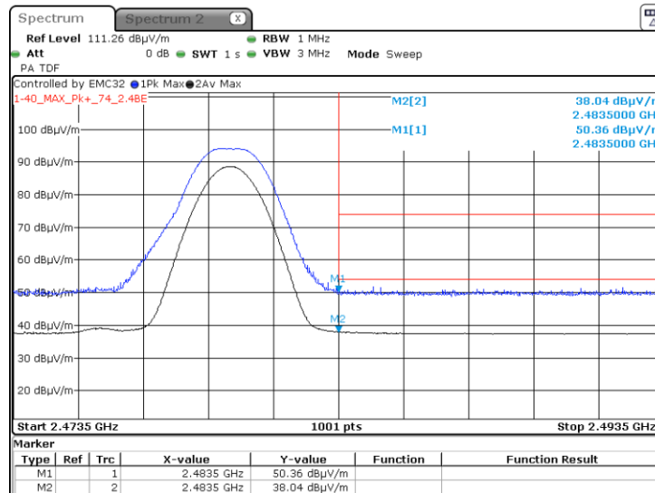
Graph 8: Radiated Upper Band Edge Plot
