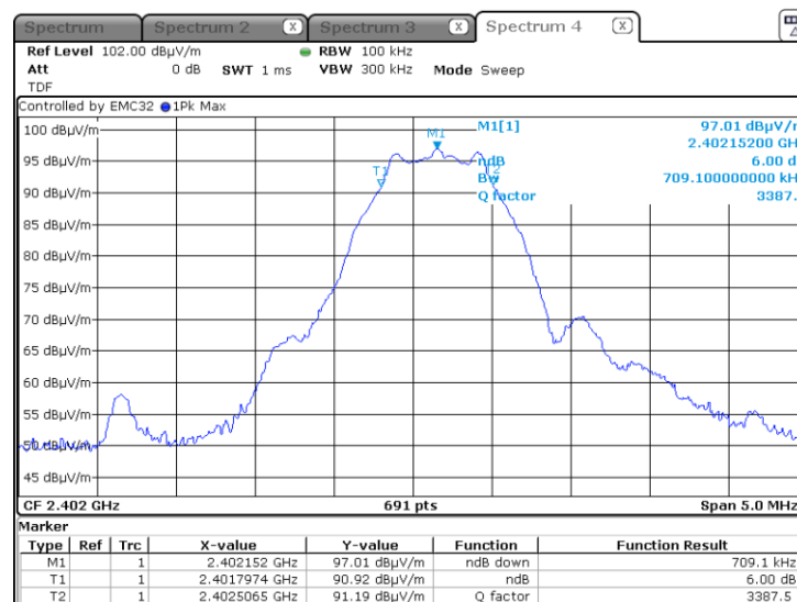
Graph 1: Lowest Channel Bandwidth
