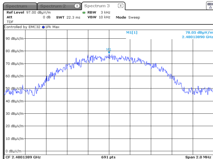
Graph 11: Highest Channel Output 3 kHz PSD Plot
