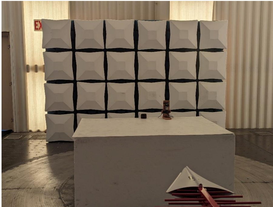
Photograph 1: Front View Radiated Emissions, 30 to 1000 MHz Worst Case Configuration
