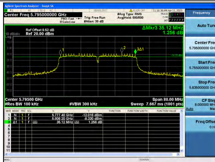
11N40SISO_Ant1_5795
