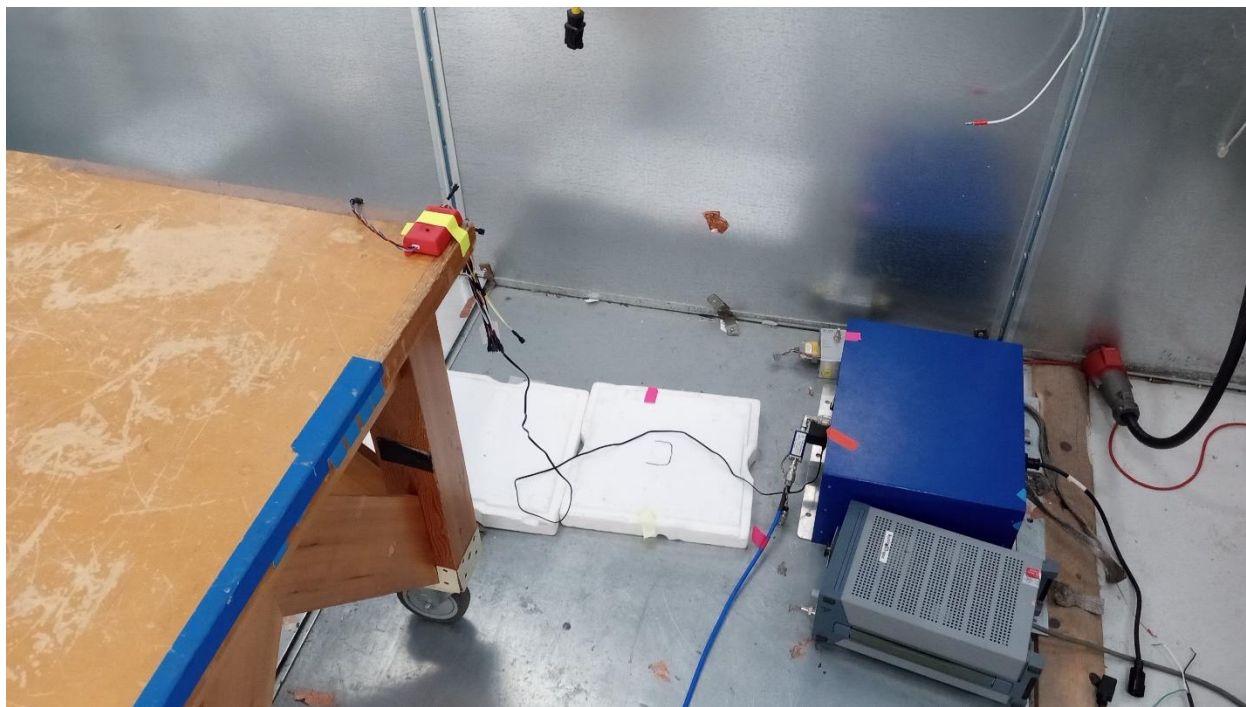
Conducted emissions Test Setup
