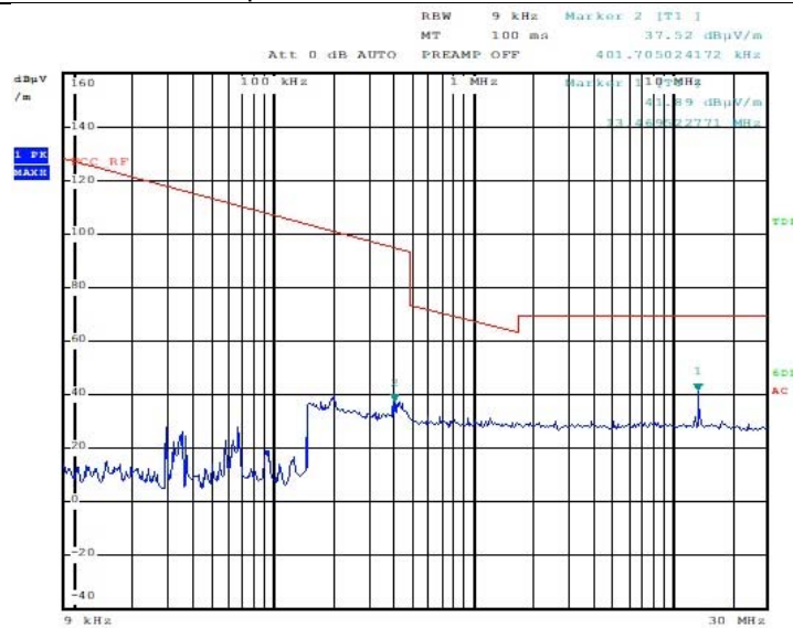
Radiated Spurious Emission 9 kHz – 30 MHz : HF ASK
