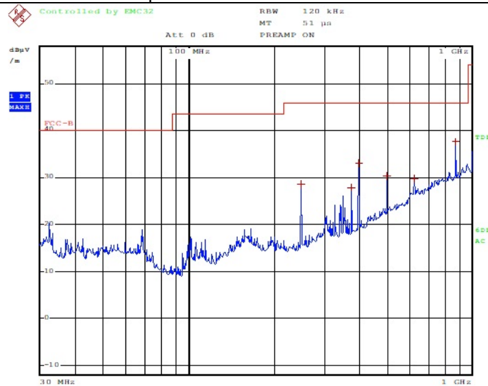
Radiated Spurious Emission 30 MHz – 1 GHz : HF ASK
