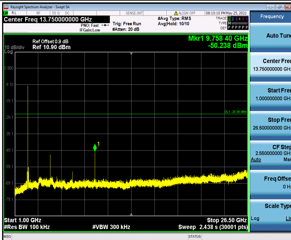
3DH5_Ant1_2441_1000~26500
