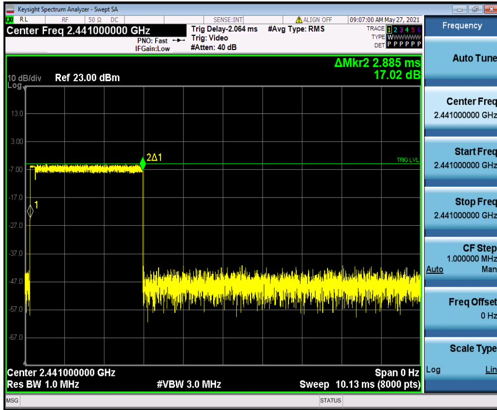
2DH5_Ant1_Hop_2441
