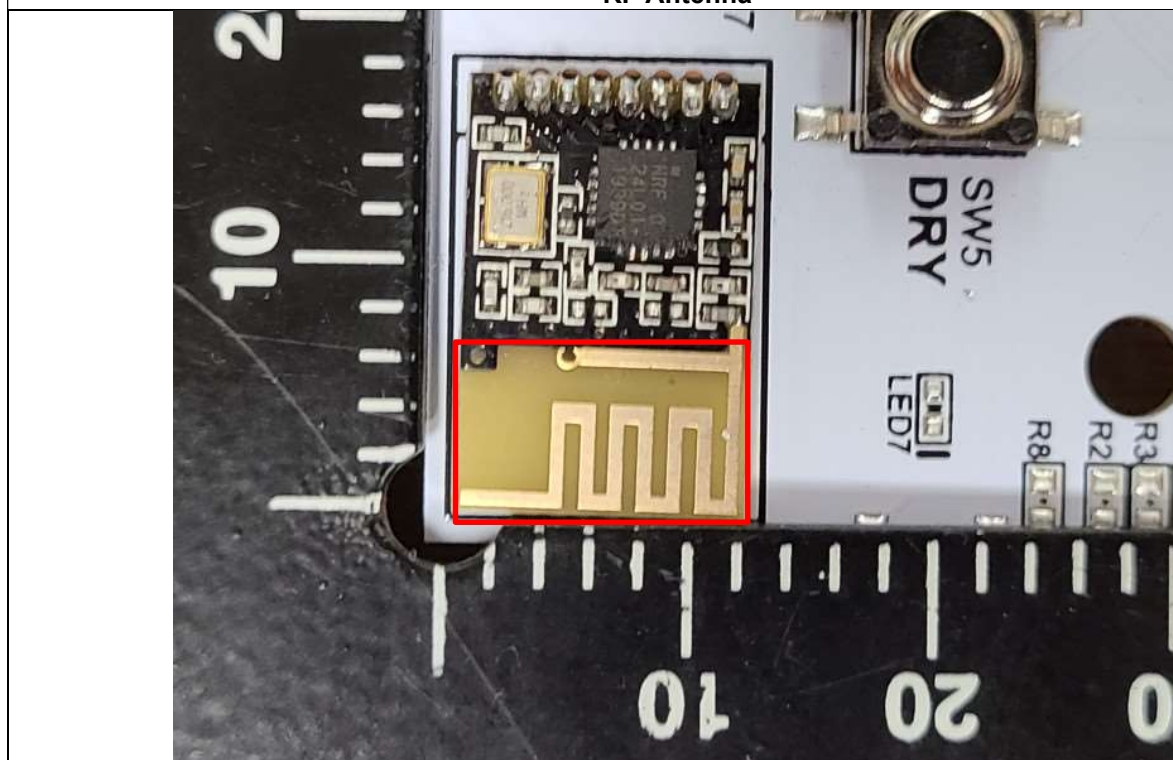
RF Antenna
