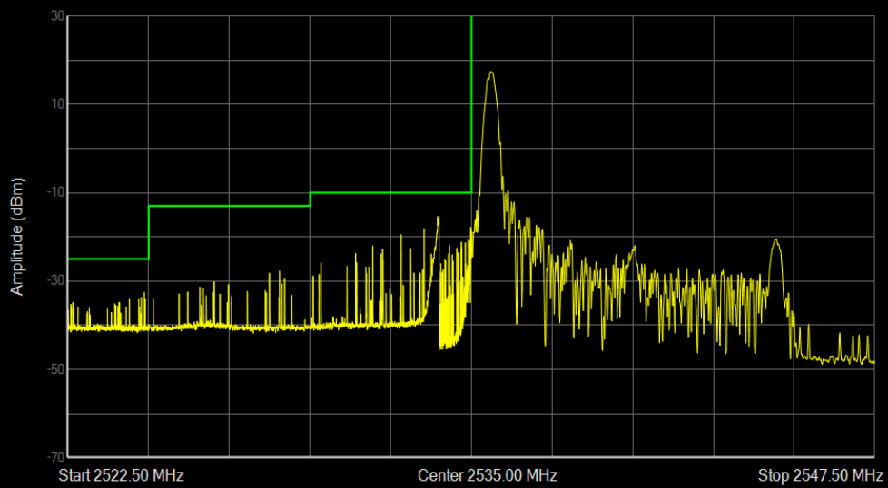
Band41(2535-2655) QPSK BW=10MHz Channel=40090 RB Size=1 Position=#0
