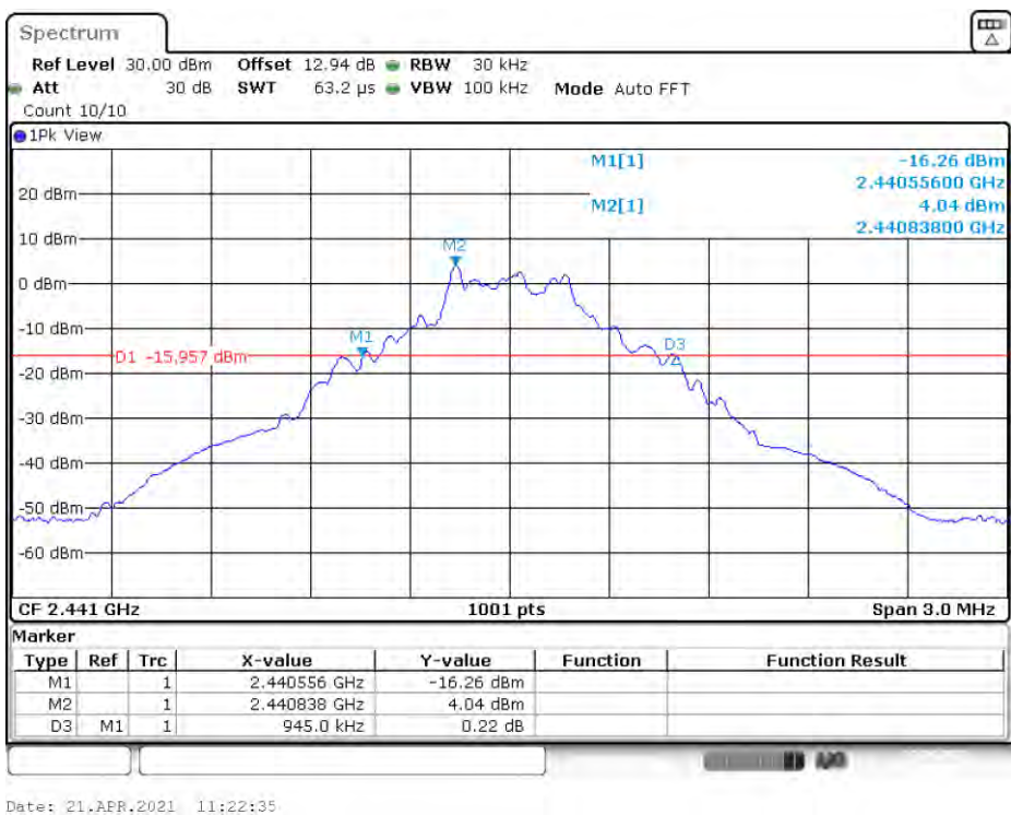
DH1_Ant1_2441MHz
