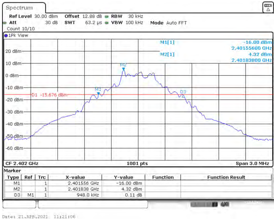
DH1_Ant1_2402MHz
