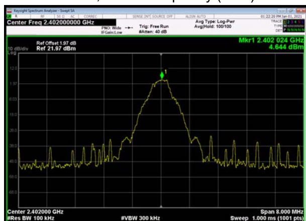
BT DH5 CH0, Carrier frequency (MHz): 2402
