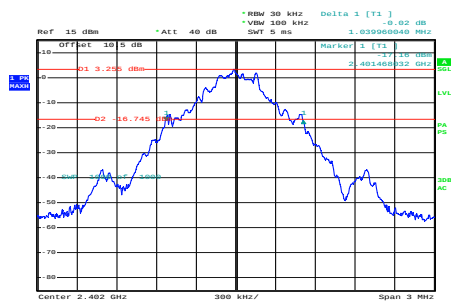
GFSK_Low
